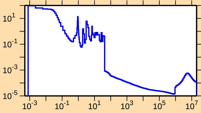
\sigma vs. E for ^{116}\text{Cs}(n,\gamma)
