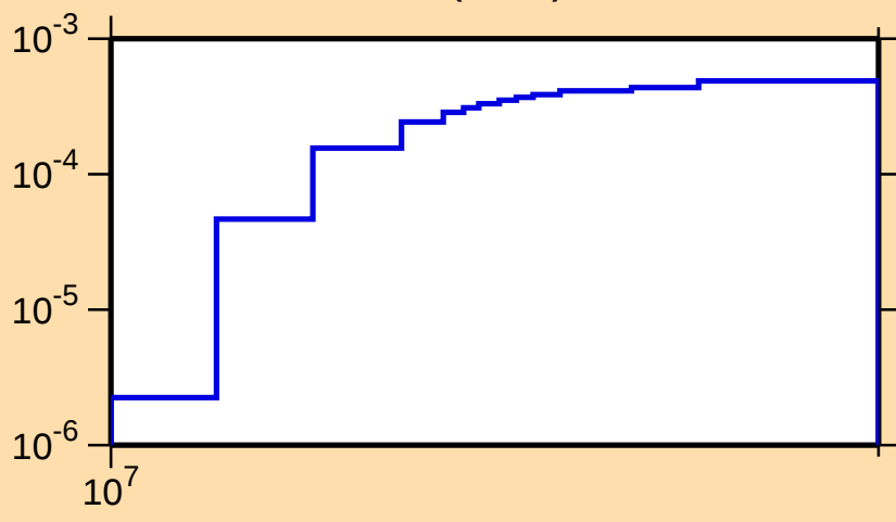
\sigma vs. E for ^{116}\text{Cs}(n,2n)
