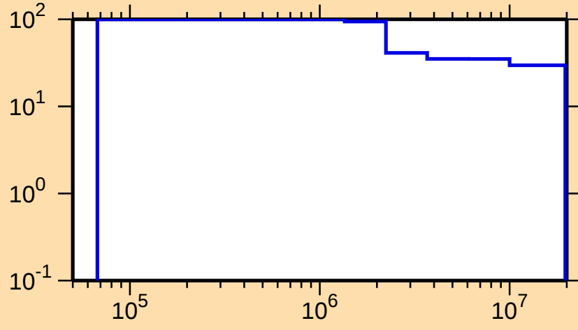
\Delta\sigma/\sigma vs. E for ^{116}\text{Cs}(n,n\text{cont.})
