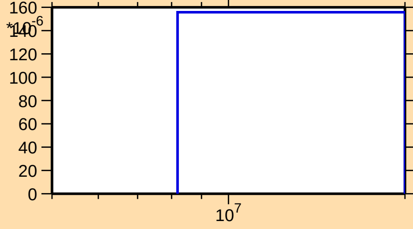
\sigma vs. E for ^{116}\text{Cs}(n,\text{pt})
