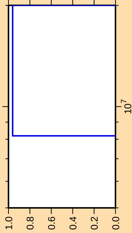
\Delta\sigma/\sigma vs. E for ^{116}\text{Cs}(n,nt)
