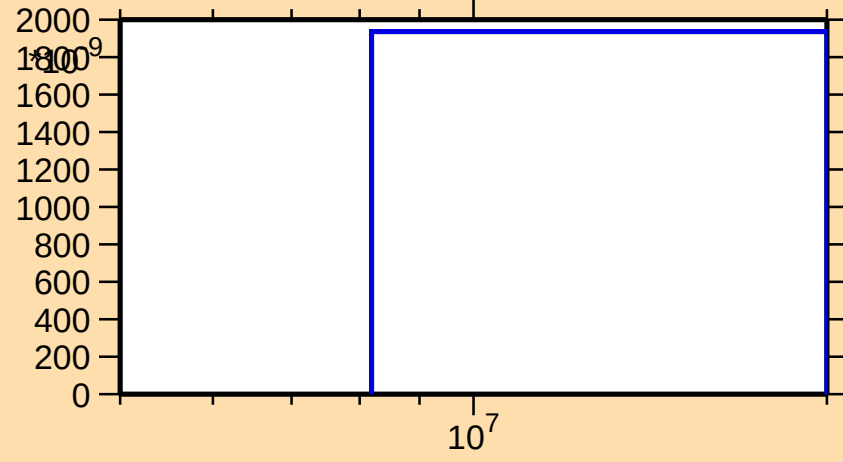
\sigma vs. E for ^{116}\text{Cs}(n,\text{nd})
