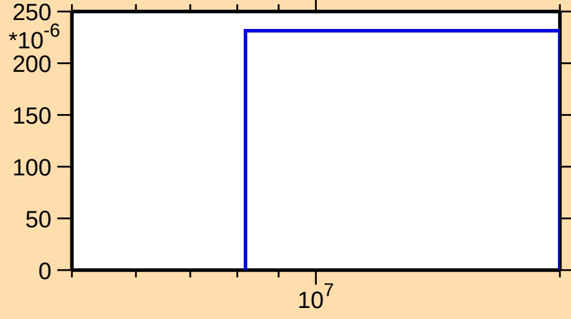
\sigma vs. E for ^{116}\text{Cs}(n,2n)
