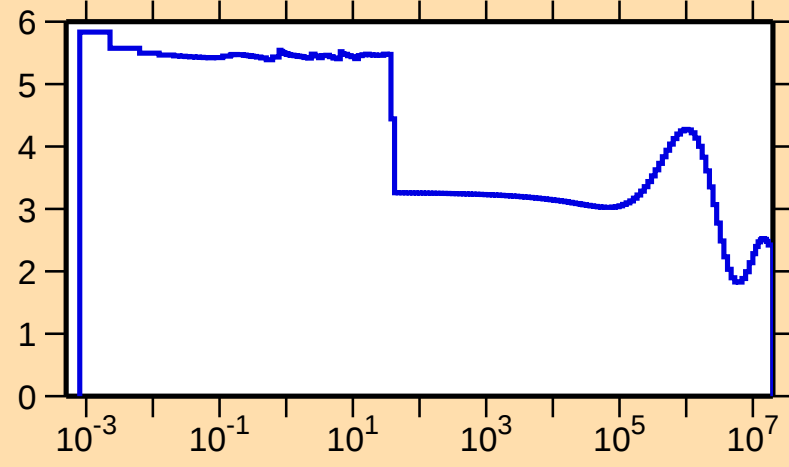
\sigma vs. E for ^{117}\text{Cs}(n,\text{el.})
