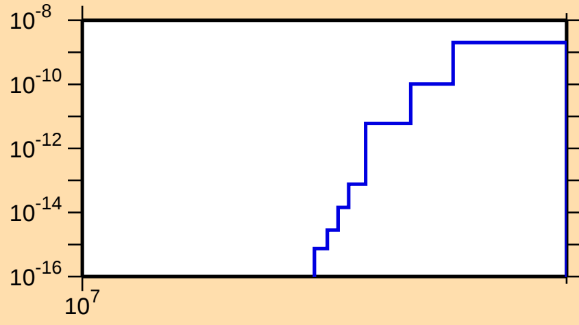
\sigma vs. E for ^{117}\text{Cs}(n,2n\alpha)
