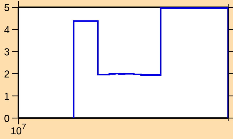
\Delta\sigma/\sigma vs. E for ^{117}\text{Cs}(n,\text{tot.})
