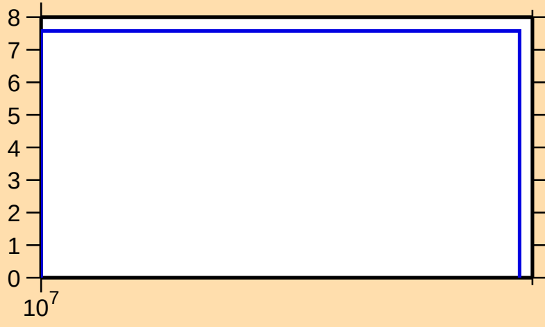
\Delta\sigma/\sigma vs. E for ^{117}\text{Cs}(n,\text{nonel.})
