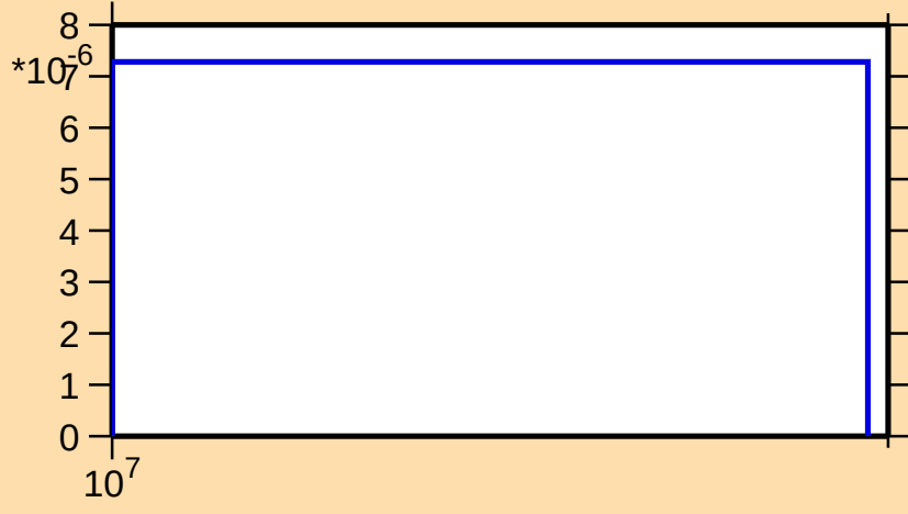
\sigma vs. E for ^{117}\text{Cs}(n,2np)
