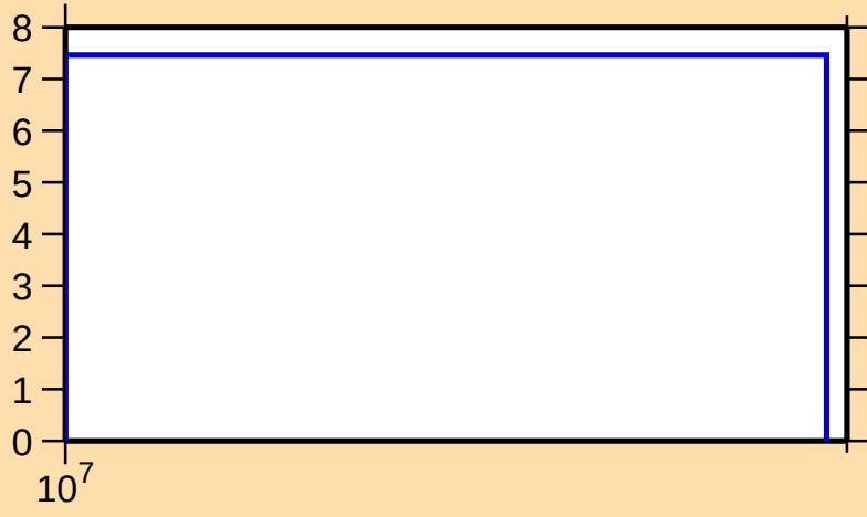
\Delta\sigma/\sigma vs. E for ^{117}\text{Cs}(n,\text{el.})
