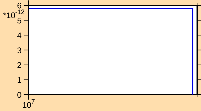
\sigma vs. E for ^{117}\text{Cs}(n,\text{nt})
