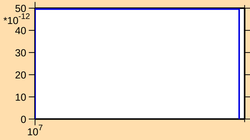
\sigma vs. E for ^{117}\text{Cs} (mt 34)
