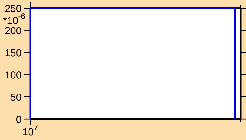
\sigma vs. E for ^{117}\text{Cs}(n,2n)
