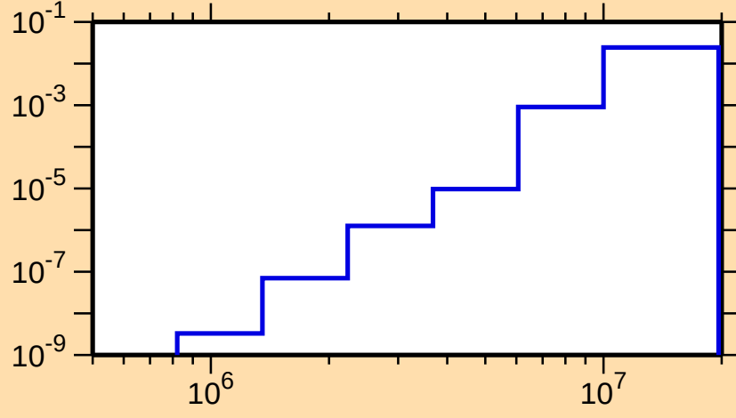
\sigma vs. E for ^{117}\text{Cs}(n,d)
