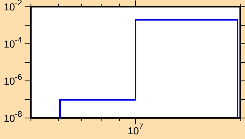
\sigma vs. E for ^{117}\text{Cs}(n,\text{pd})
