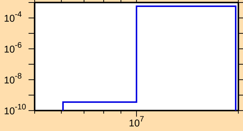
\sigma vs. E for ^{117}\text{Cs}(n,t)
