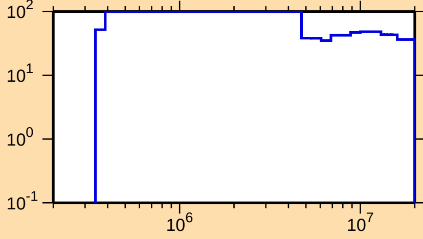
\Delta\sigma/\sigma vs. E for ^{118}\text{Cs}(n,n\text{cont.})
