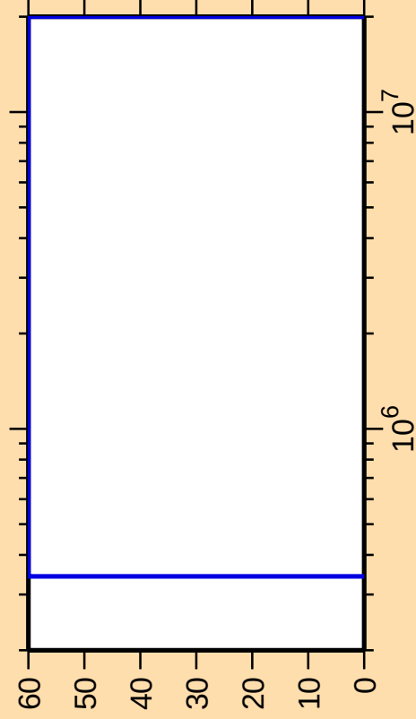
\Delta\sigma/\sigma vs. E for ^{118}\text{Cs}(n,\alpha)
