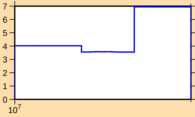
\Delta\sigma/\sigma vs. E for ^{118}\text{Cs}(n,\text{tot.})
