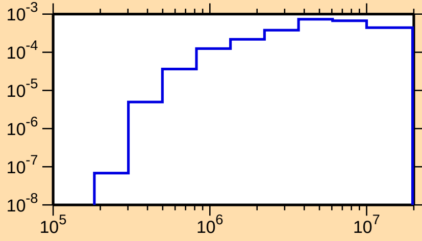
\sigma vs. E for ^{118}\text{Cs}(n,n_4)
