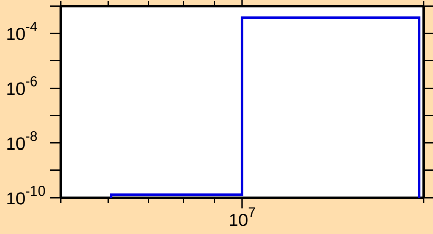
\sigma vs. E for ^{118}\text{Cs}(n,\text{pd})
