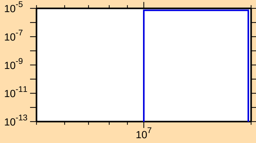
\sigma vs. E for ^{118}\text{Cs}(n,\text{nd})
