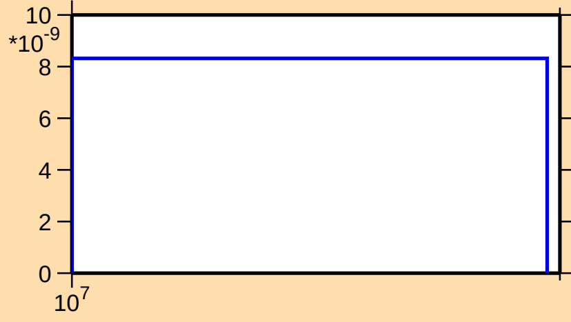
\sigma vs. E for ^{118}\text{Cs} (mt 34)
