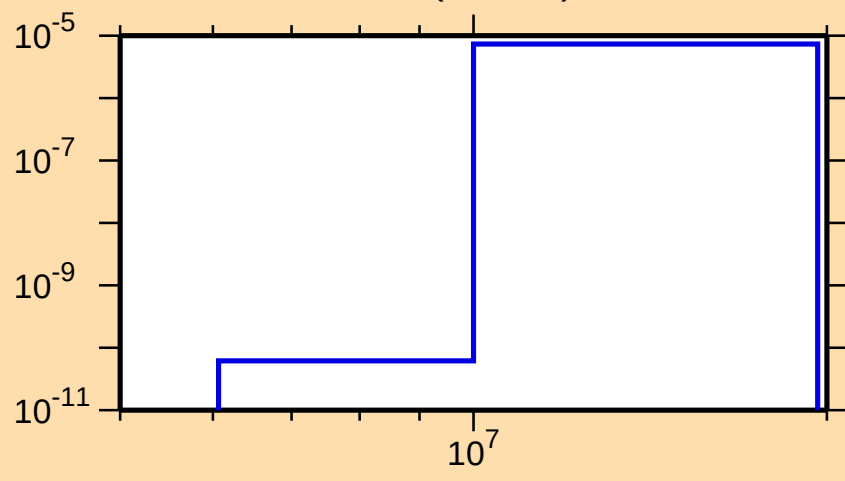
\sigma vs. E for ^{118}\text{Cs}(\text{mt117})
