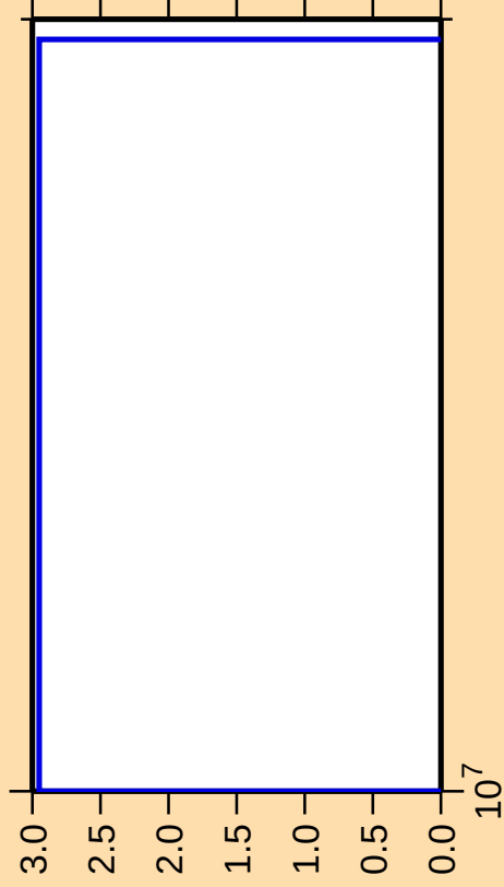
\Delta\sigma/\sigma vs. E for ^{118}\text{Cs}(n,nt)
