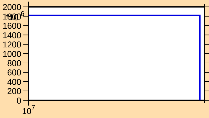
\sigma vs. E for ^{118}\text{Cs}(n,2n)
