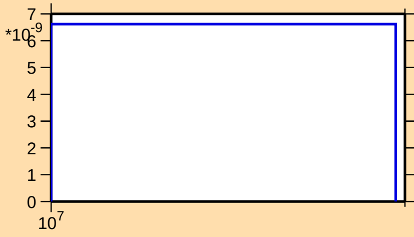
\sigma vs. E for ^{118}\text{Cs}(n,2n\alpha)
