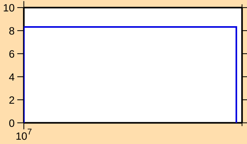
\Delta\sigma/\sigma vs. E for ^{118}\text{Cs}(n,\text{el.})
