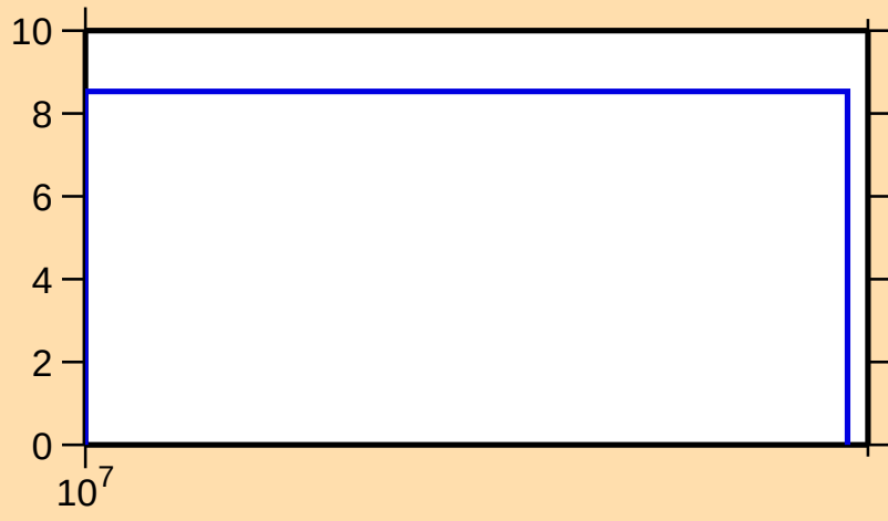
\Delta\sigma/\sigma vs. E for ^{118}\text{Cs}(n,\text{nonel.})
