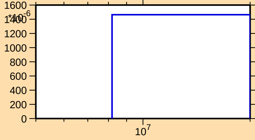
\sigma vs. E for ^{118}\text{Cs}(n,2n)
