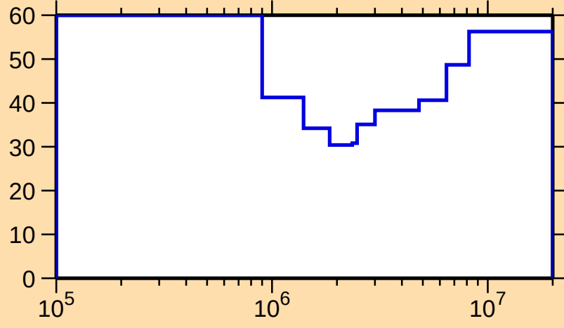
\Delta\sigma/\sigma vs. E for ^{118}\text{Cs}(n,n_1)
