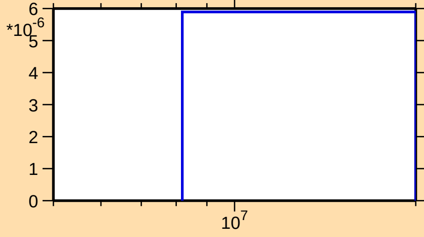
\sigma vs. E for ^{118}\text{Cs}(n,\text{nd})
