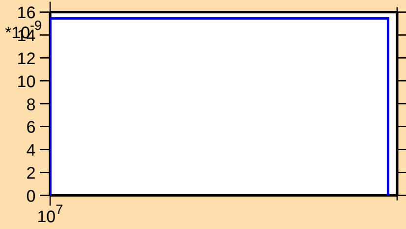
\sigma vs. E for ^{118}\text{Cs}(\text{mt } 34)
