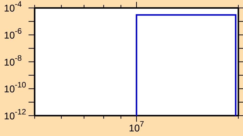
\sigma vs. E for ^{118}\text{Cs}(n,\text{pt})
