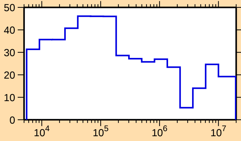
\Delta\sigma/\sigma vs. E for ^{118}\text{Cs}(n,\text{tot.})
