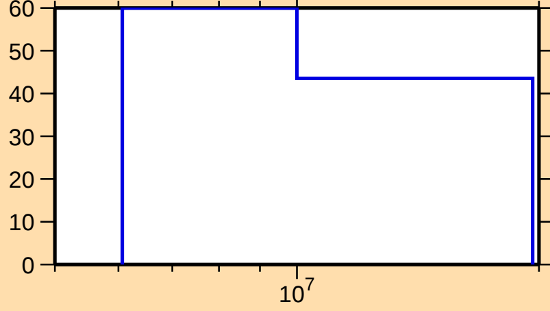
\Delta\sigma/\sigma vs. E for ^{118}\text{Cs}(n,\text{el.})
