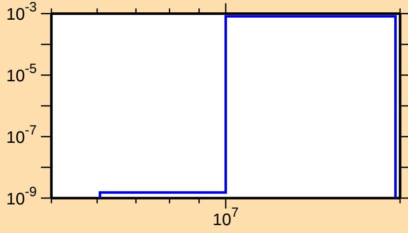
\sigma vs. E for ^{118}\text{Cs}(n,\text{pd})
