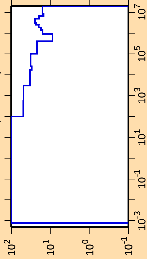
\Delta\sigma/\sigma vs. E for ^{118}\text{Cs}(n,\text{nonel.})
