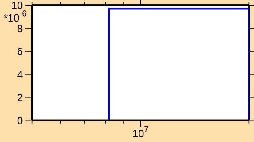
\sigma vs. E for ^{118}\text{Cs}(n,nd)
