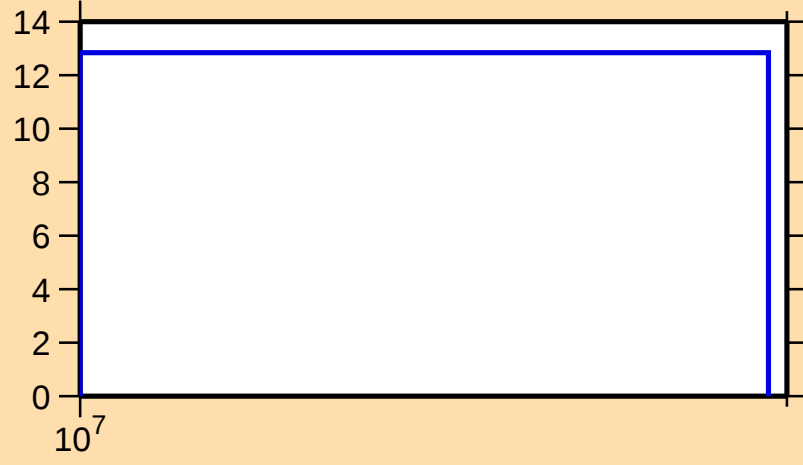
\Delta\sigma/\sigma vs. E for ^{119}\text{Cs}(n,\text{tot.})
