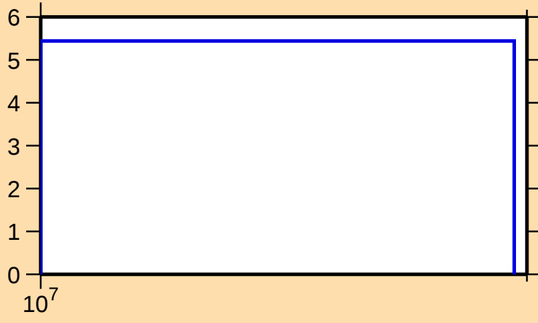
\Delta\sigma/\sigma vs. E for ^{119}\text{Cs}(n,\text{nonel.})
