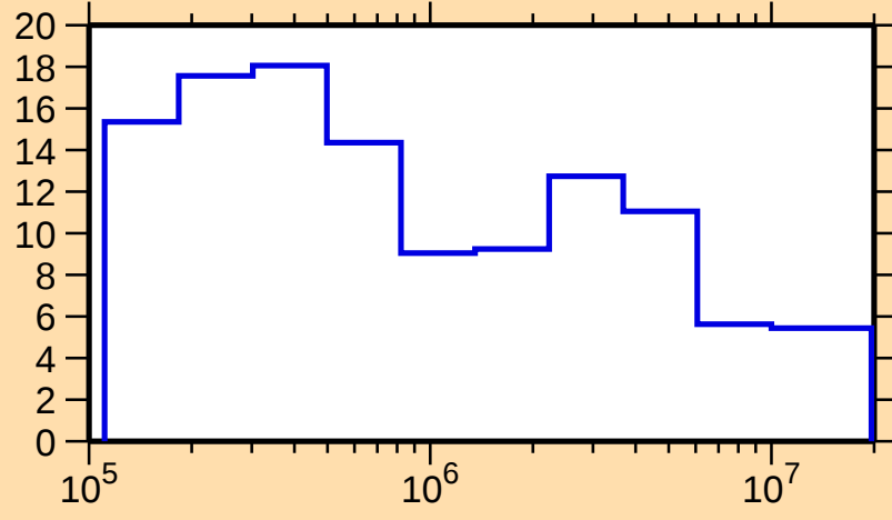
\Delta\sigma/\sigma vs. E for ^{119}\text{Cs}(n,\text{nonel.})
