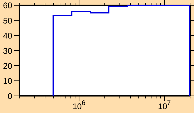
\Delta\sigma/\sigma vs. E for ^{119}\text{Cs}(n,n_1)
