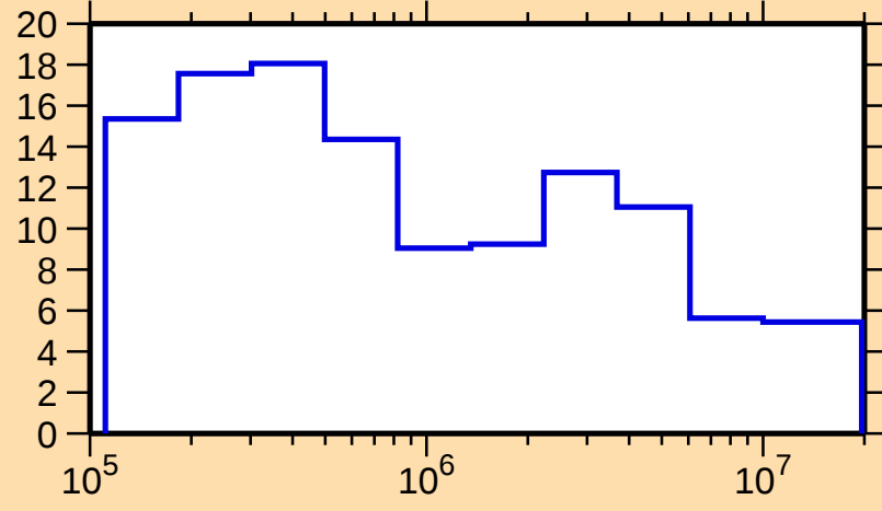
\Delta\sigma/\sigma vs. E for ^{119}\text{Cs}(n,\text{nonel.})
