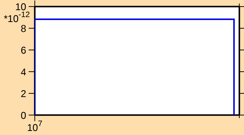
\sigma vs. E for ^{119}\text{Cs}(n,nt)
