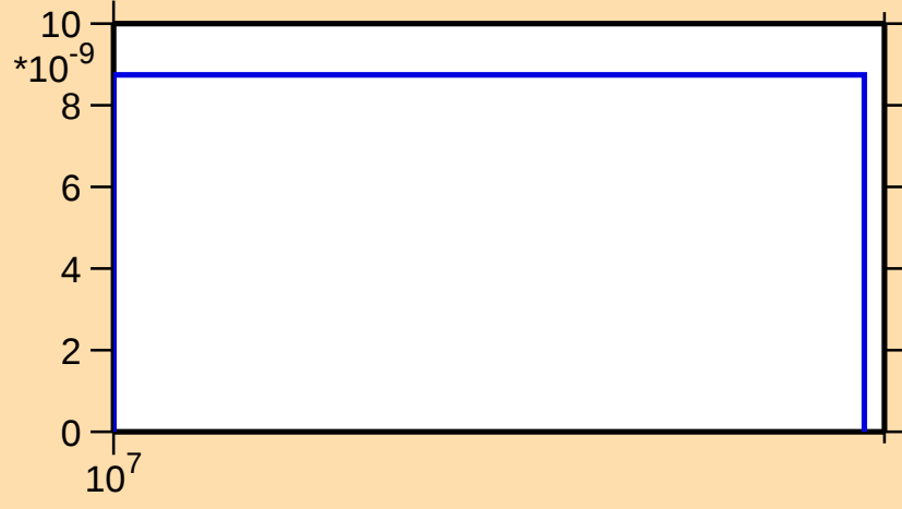
\sigma vs. E for ^{119}\text{Cs}(n,\text{pt})
