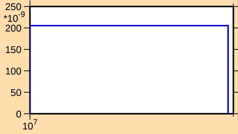
\sigma vs. E for ^{119}\text{Cs}(n,\text{nd})
