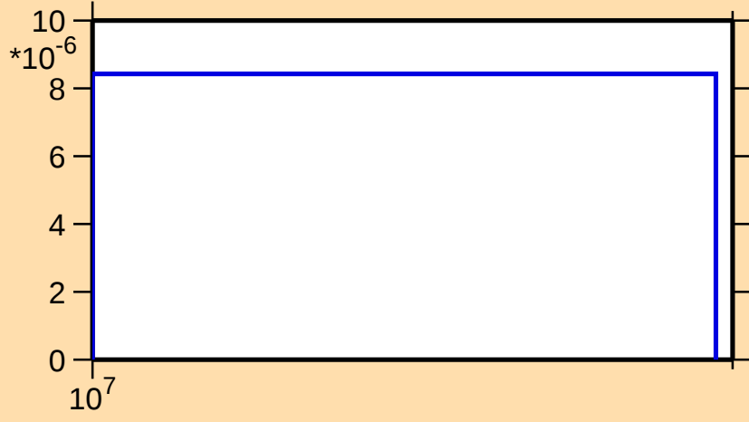
\sigma vs. E for ^{119}\text{Cs}(n,2np)
