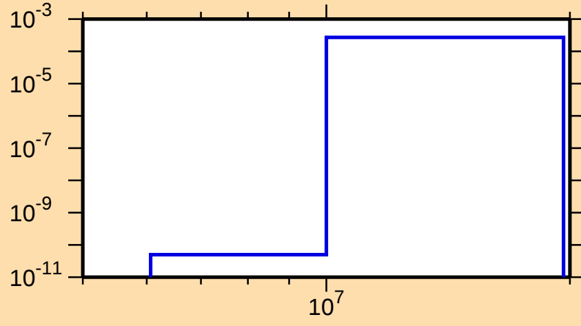
\sigma vs. E for ^{119}\text{Cs}(n,t)
