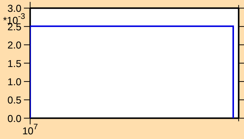
\sigma vs. E for ^{119}\text{Cs}(n,2n)
