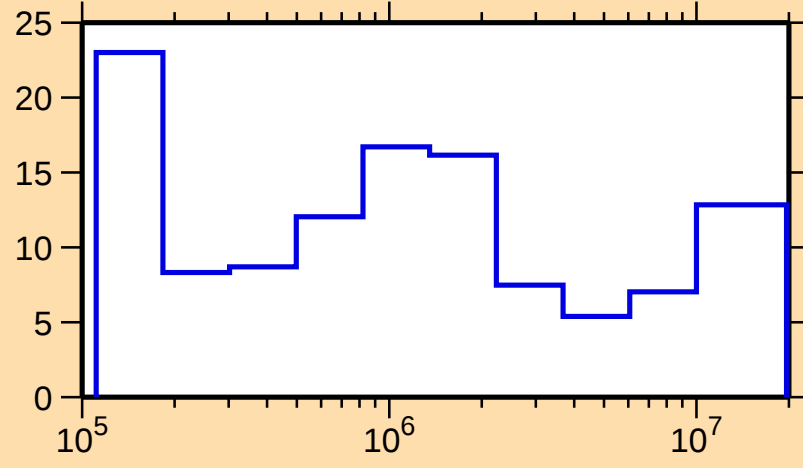
\Delta\sigma/\sigma vs. E for ^{119}\text{Cs}(n,\text{tot.})
