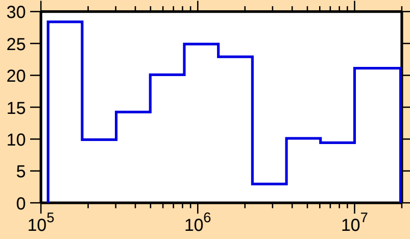
\Delta\sigma/\sigma vs. E for ^{119}\text{Cs}(n,\text{el.})
