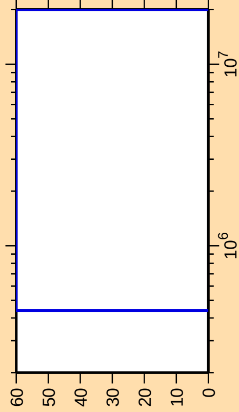
\Delta\sigma/\sigma vs. E for ^{120}\text{Cs}(n,n_{\text{cont}})
