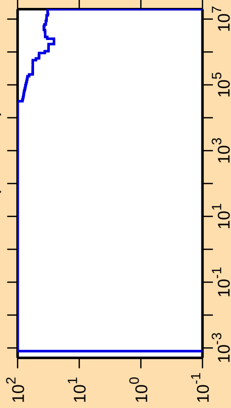
\Delta\sigma/\sigma vs. E for ^{120}\text{Cs}(n,\text{nonel.})
