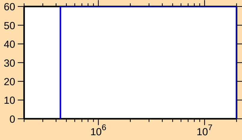
\Delta\sigma/\sigma vs. E for ^{120}\text{Cs}(n,n_1)
