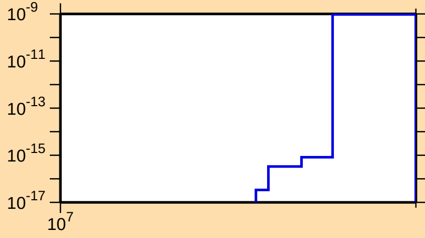
\sigma vs. E for ^{120}\text{Cs}(n,nt)
