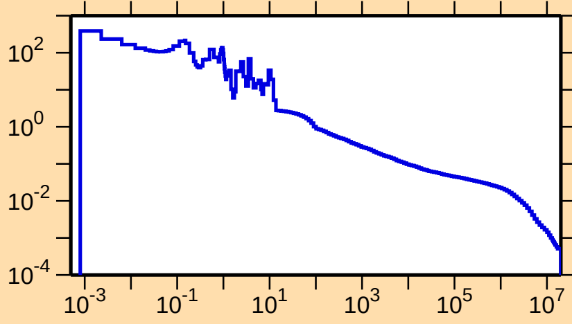
\sigma vs. E for ^{120}\text{Cs}(n,\gamma)
