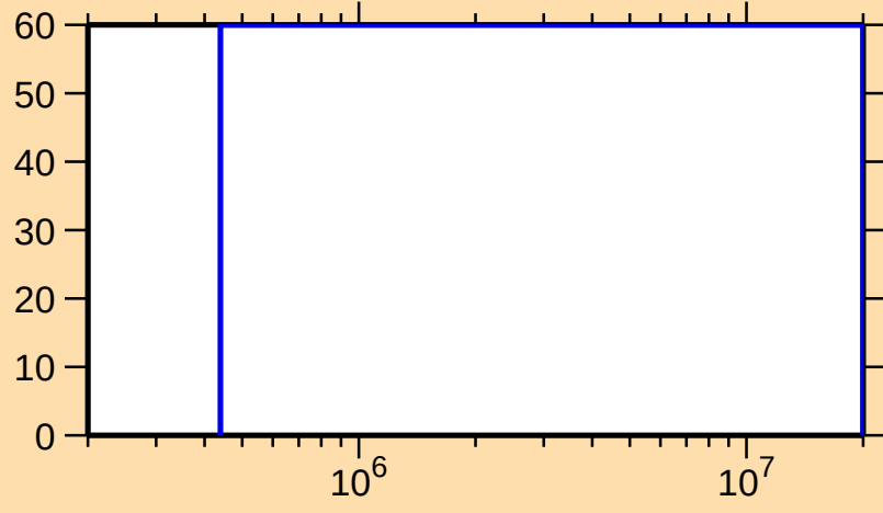
\Delta\sigma/\sigma vs. E for ^{120}\text{Cs}(n,n\text{cont.})
