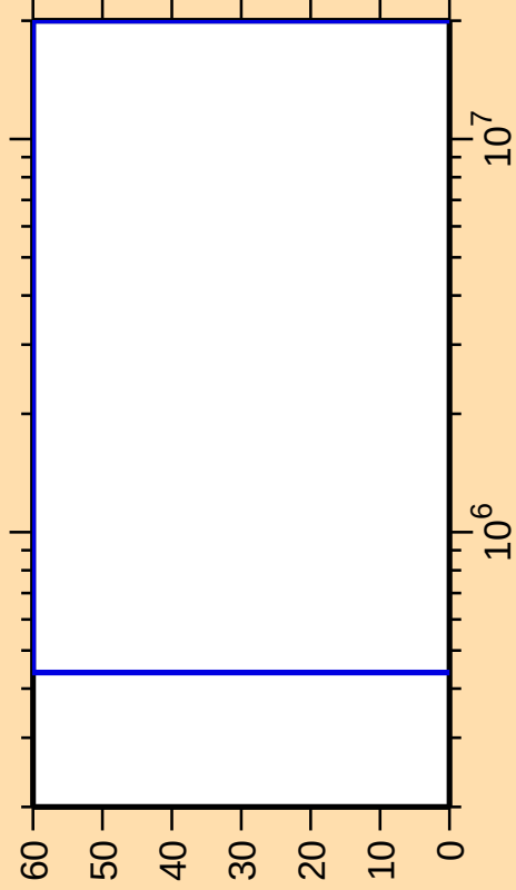
\Delta\sigma/\sigma vs. E for ^{120}\text{Cs}(n,\alpha)
