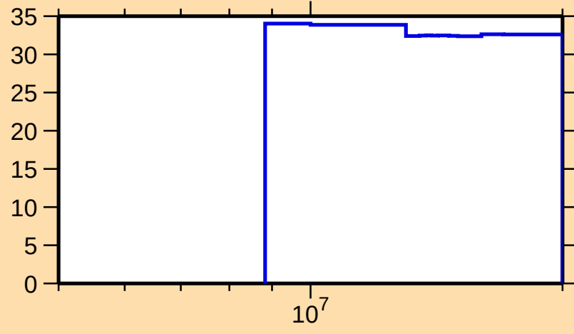
\Delta\sigma/\sigma vs. E for ^{120}\text{Cs}(n,\text{nonel.})
