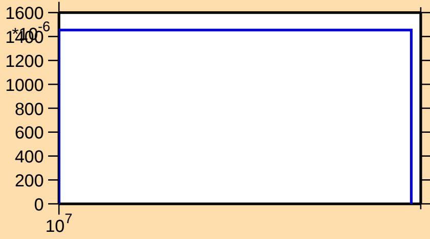
\sigma vs. E for ^{120}\text{Cs}(n,2np)
