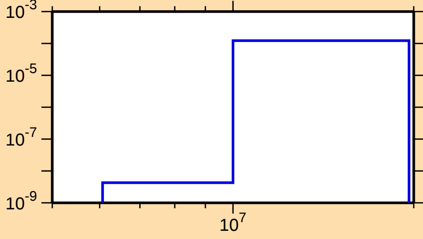
\sigma vs. E for ^{120}\text{Cs}(n,\text{He}3)
