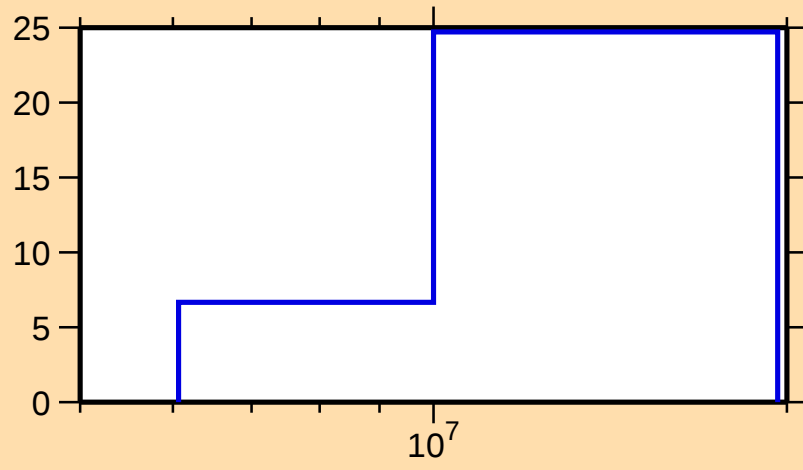
\Delta\sigma/\sigma vs. E for ^{120}\text{Cs}(n,\text{tot.})
