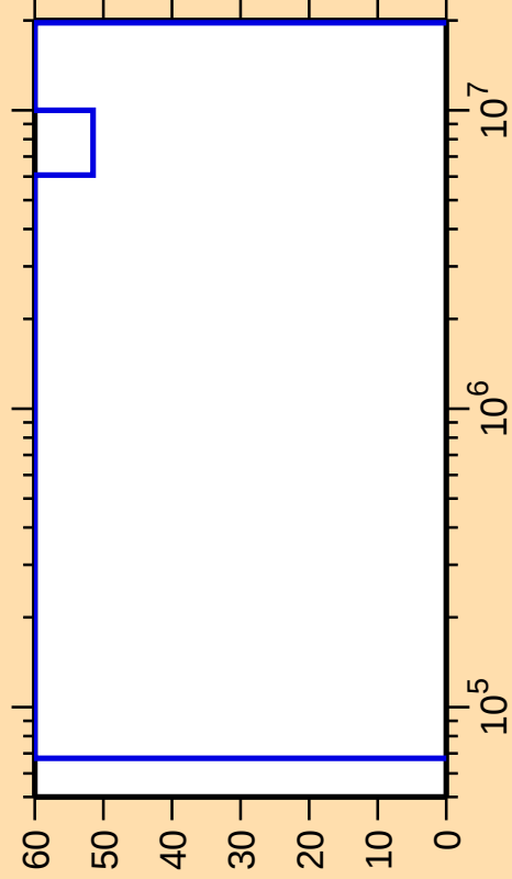
\Delta\sigma/\sigma vs. E for ^{120}\text{Cs}(n,\text{inel.})
