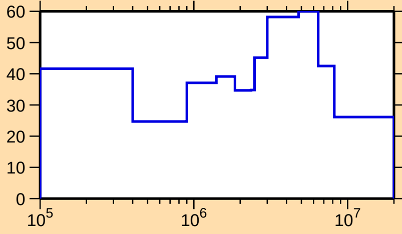
\Delta\sigma/\sigma vs. E for ^{120}\text{Cs}(n,\text{el.})
