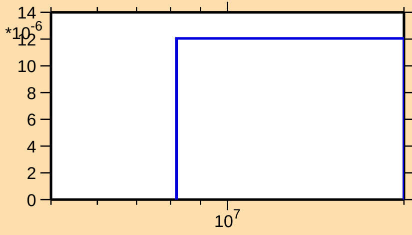
\sigma vs. E for ^{120}\text{Cs}(\text{mt } 45)
