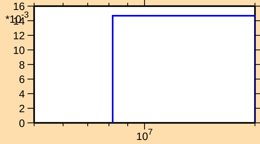
\sigma vs. E for ^{120}\text{Cs}(n,2n)
