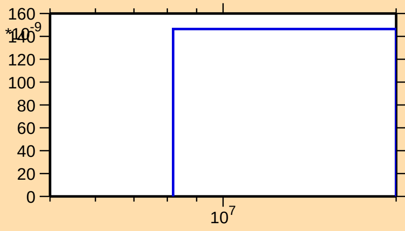
\sigma vs. E for ^{120}\text{Cs}(\text{mt117})
