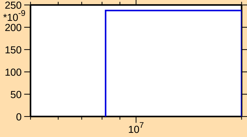
\sigma vs. E for ^{120}\text{Cs}(n,\text{pt})
