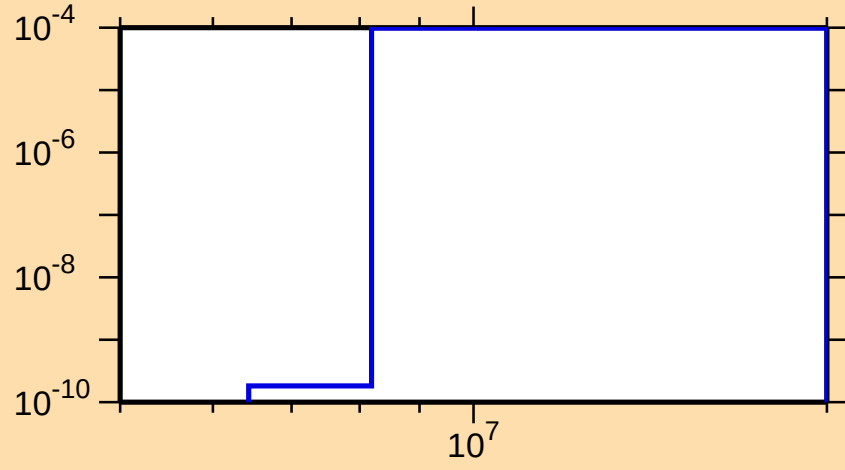
\sigma vs. E for ^{120}\text{Cs}(n,\text{He}3)
