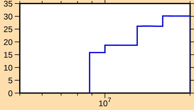
\Delta\sigma/\sigma vs. E for ^{120}\text{Cs}(n,\text{tot.})
