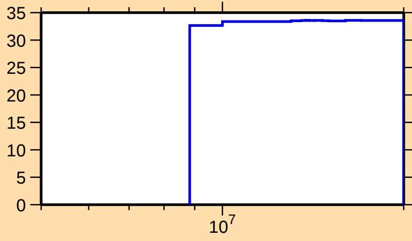
\Delta\sigma/\sigma vs. E for ^{120}\text{Cs}(n,\text{nonel.})
