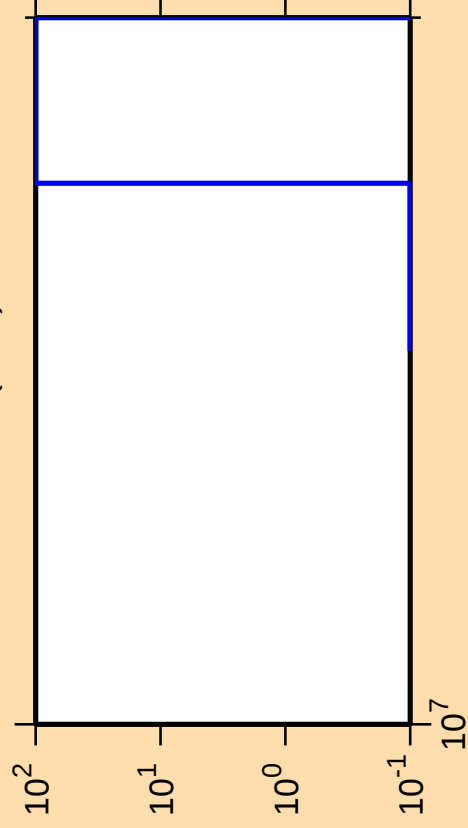
\Delta\sigma/\sigma vs. E for ^{120}\text{Cs}(n,nt)
