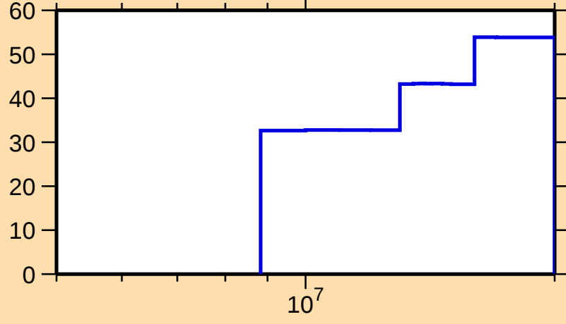
\Delta\sigma/\sigma vs. E for ^{120}\text{Cs}(n,\text{el.})
