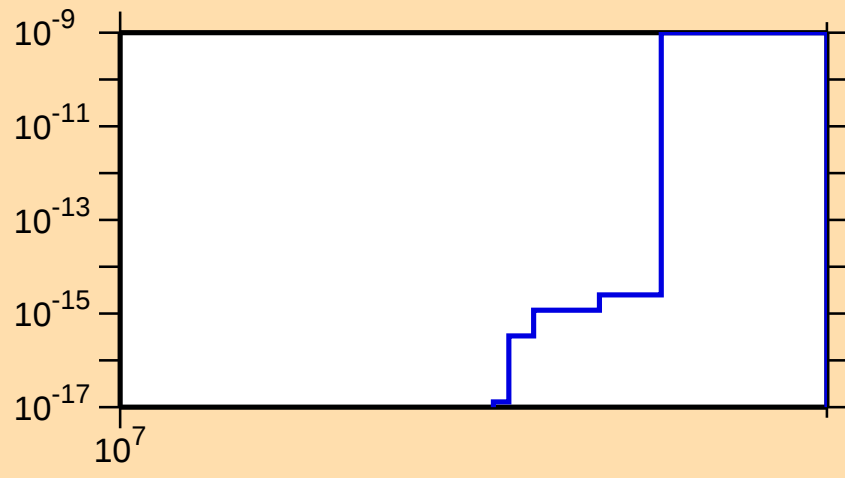
\sigma vs. E for ^{120}\text{Cs}(n,nt)
