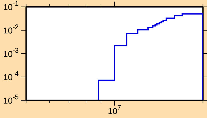
\sigma vs. E for ^{120}\text{Cs}(n,2n)
