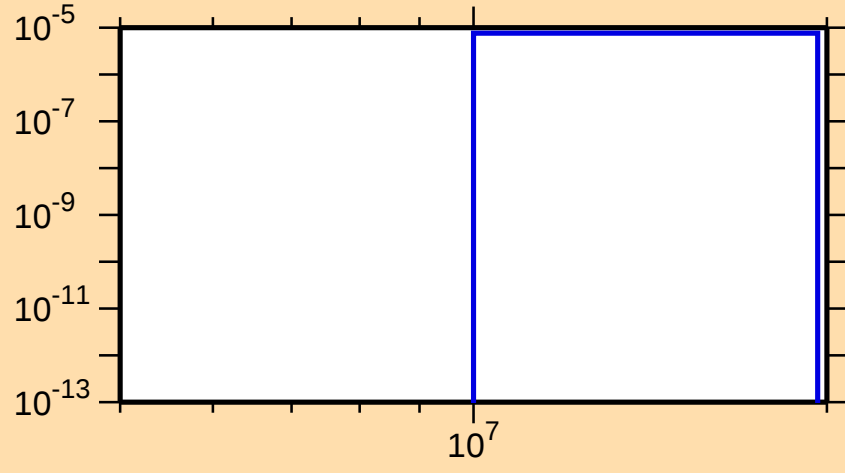
\sigma vs. E for ^{120}\text{Cs}(n,\text{nd})
