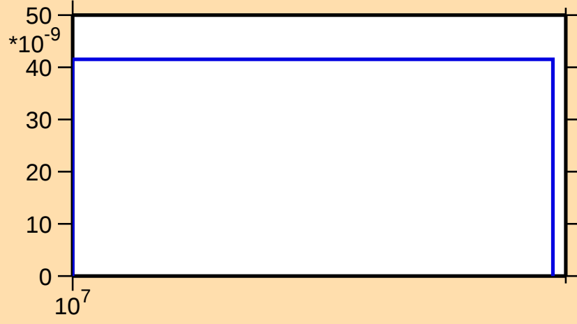
\sigma vs. E for ^{120}\text{Cs}(n,2n\alpha)
