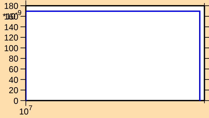
\sigma vs. E for ^{120}\text{Cs}(n,\text{pt})
