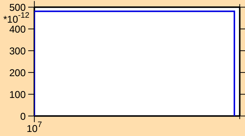
\sigma vs. E for ^{120}\text{Cs} (mt 34)
