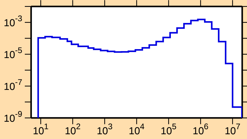
\sigma vs. E for ^{120}\text{Cs}(n,n_2)
