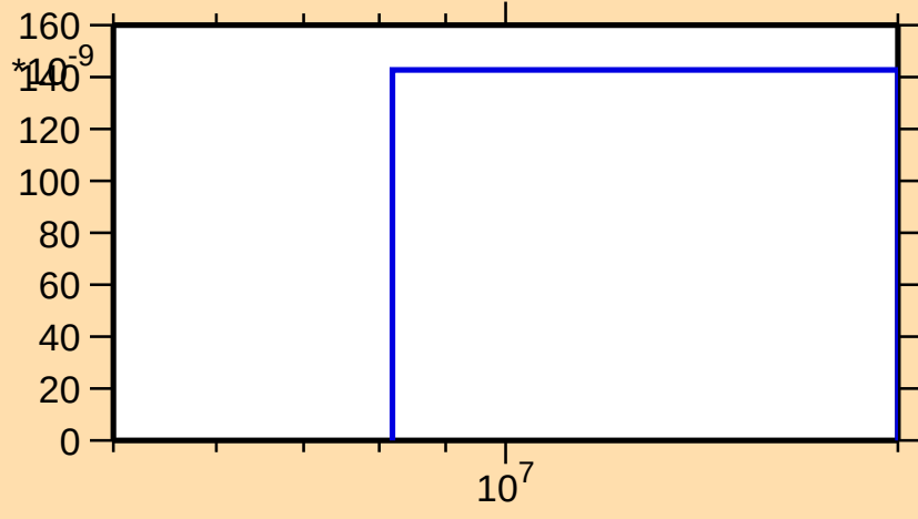
\sigma vs. E for ^{120}\text{Cs}(n,pt)
