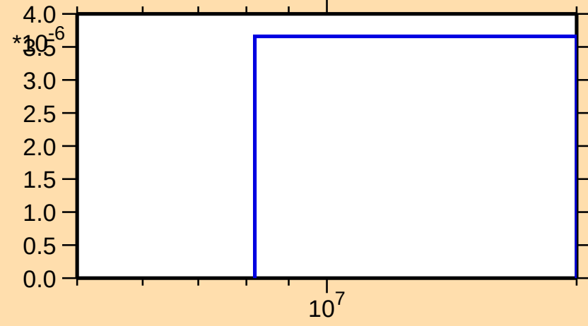
\sigma vs. E for ^{120}\text{Cs}(n,\text{pd})
