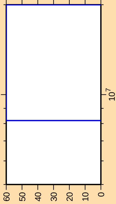
\Delta\sigma/\sigma vs. E for ^{120}\text{Cs}(n,pt)
