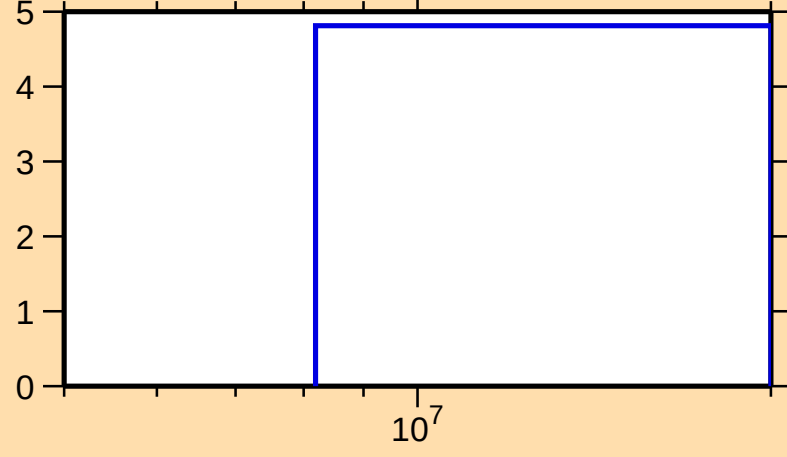
\Delta\sigma/\sigma vs. E for ^{121}\text{Cs}(n,\text{nonel.})
