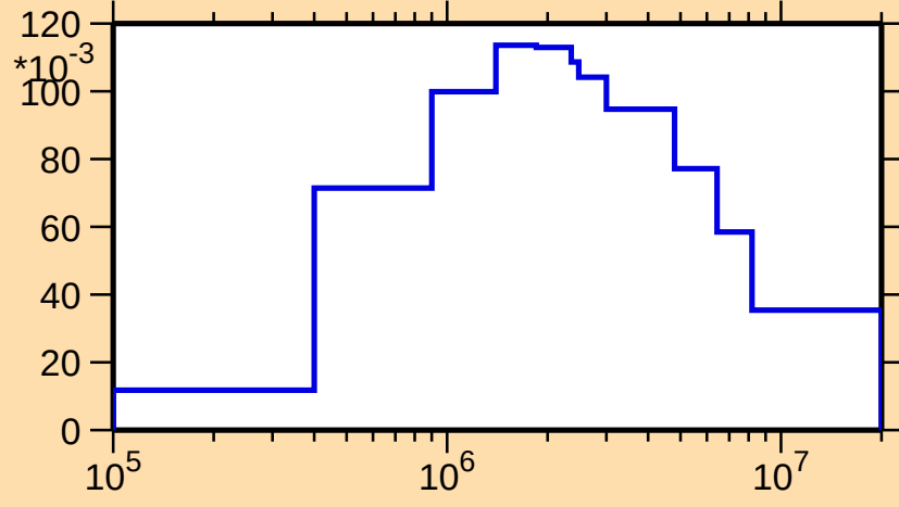
\sigma vs. E for ^{121}\text{Cs}(n,n_4)
