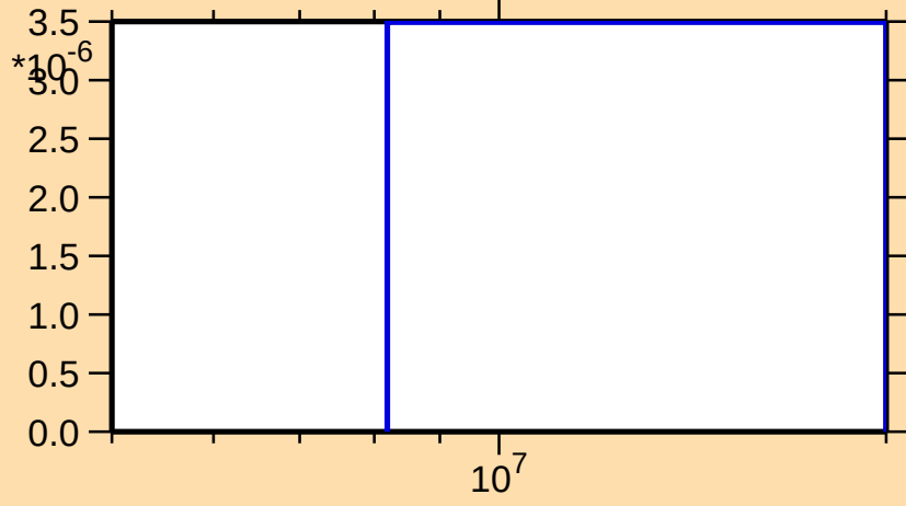
\sigma vs. E for ^{121}\text{Cs}(n,\text{pd})
