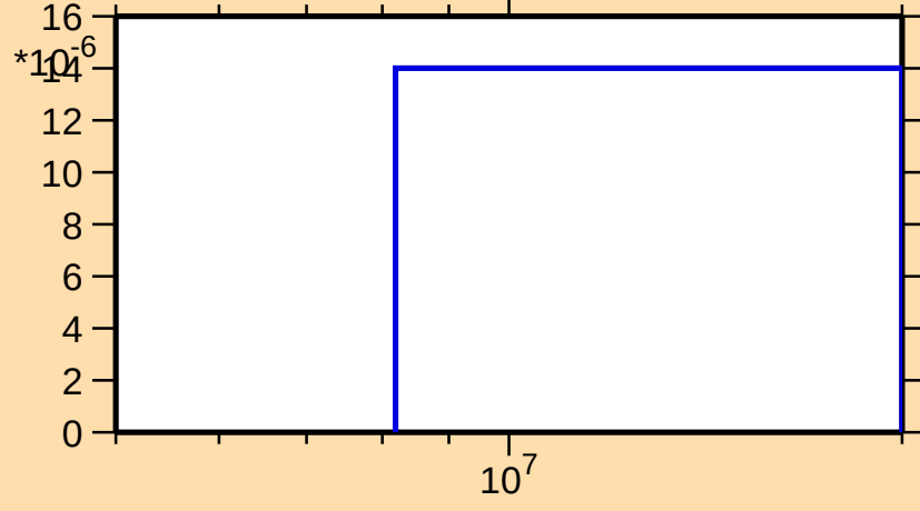
\sigma vs. E for ^{121}\text{Cs}(n,2np)
