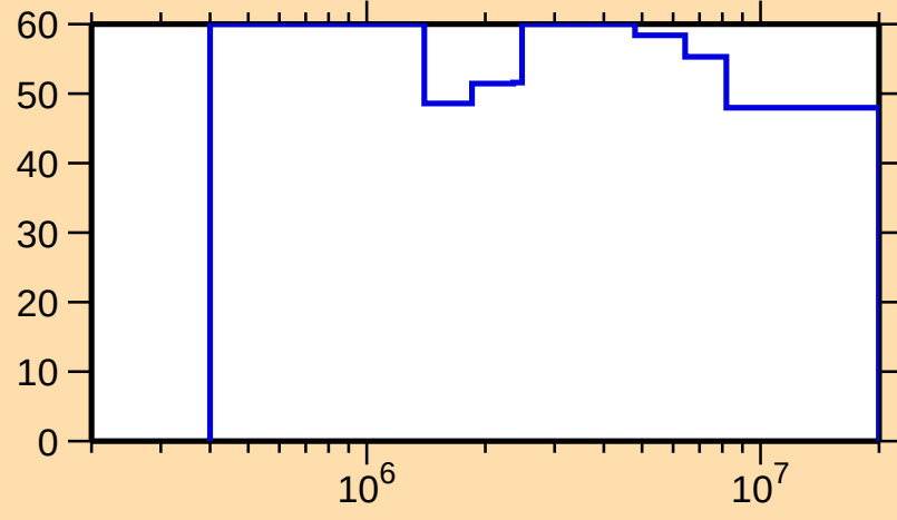
\Delta\sigma/\sigma vs. E for ^{121}\text{Cs}(n,n_1)
