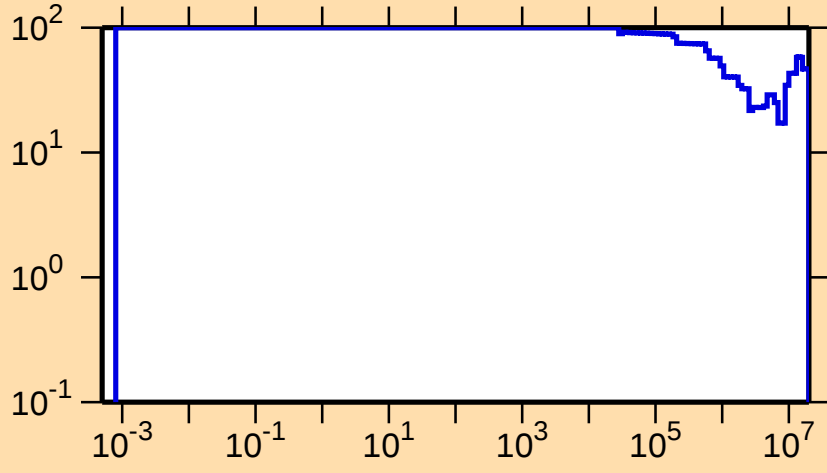
\Delta\sigma/\sigma vs. E for ^{121}\text{Cs}(n,p)
