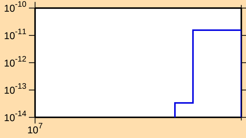
\sigma vs. E for ^{121}\text{Cs} (mt 34)
