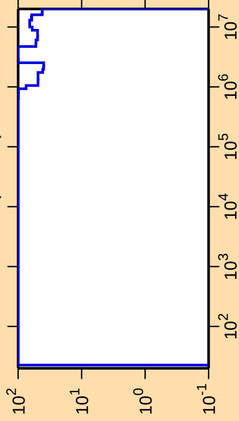
\Delta\sigma/\sigma vs. E for ^{121}\text{Cs}(n,\text{inel.})
