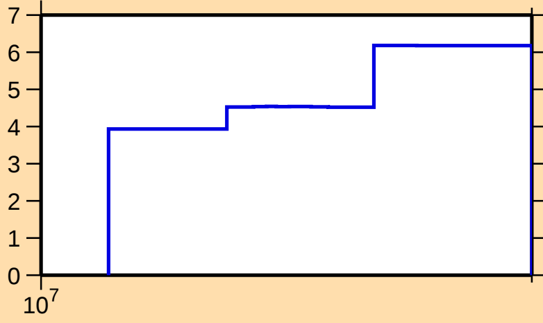
\Delta\sigma/\sigma vs. E for ^{121}\text{Cs}(n,\text{tot.})
