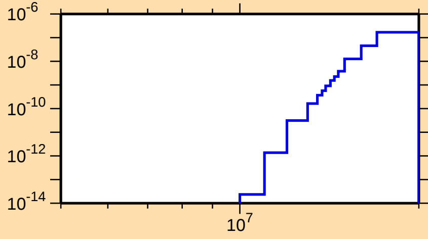
\sigma vs. E for ^{122}\text{Cs}(\text{mt117})
