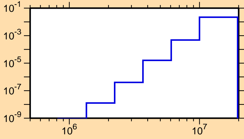
\sigma vs. E for ^{122}\text{Cs}(n,p\alpha)
