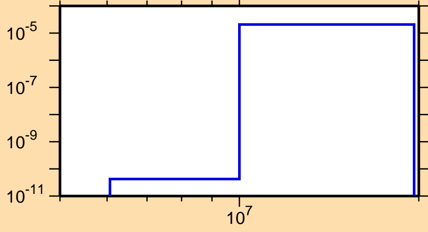
\sigma vs. E for ^{122}\text{Cs}(n,\text{He}3)
