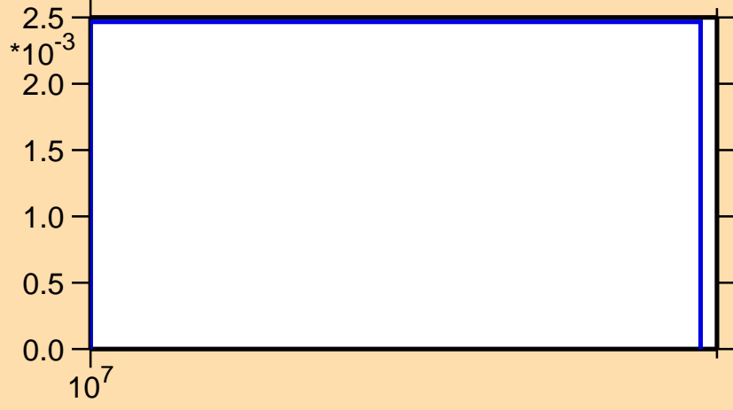
\sigma vs. E for ^{122}\text{Cs}(n,2np)
