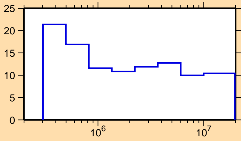
\Delta\sigma/\sigma vs. E for ^{122}\text{Cs}(n, \text{el.})
