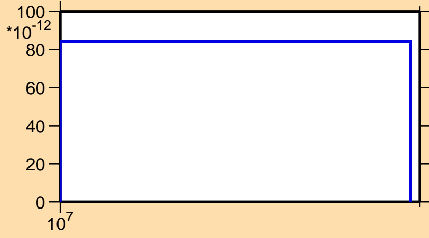
\sigma vs. E for ^{122}\text{Cs} (mt 34)
