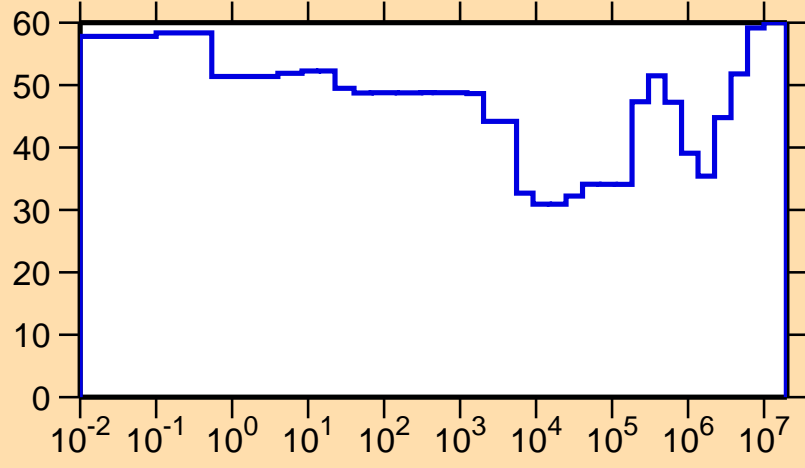
\Delta\sigma/\sigma vs. E for ^{122}\text{Cs}(n,p)
