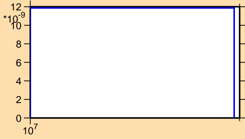
\sigma vs. E for ^{122}\text{Cs}(n,\text{pt})
