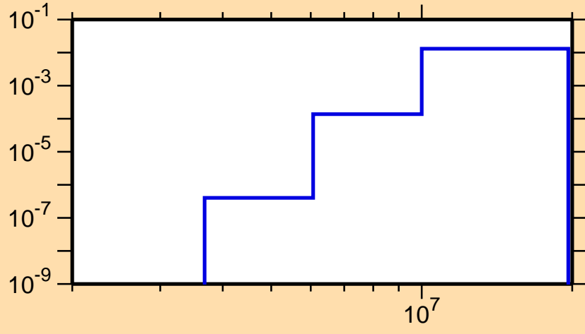
\sigma vs. E for ^{122}\text{Cs}(n,d)
