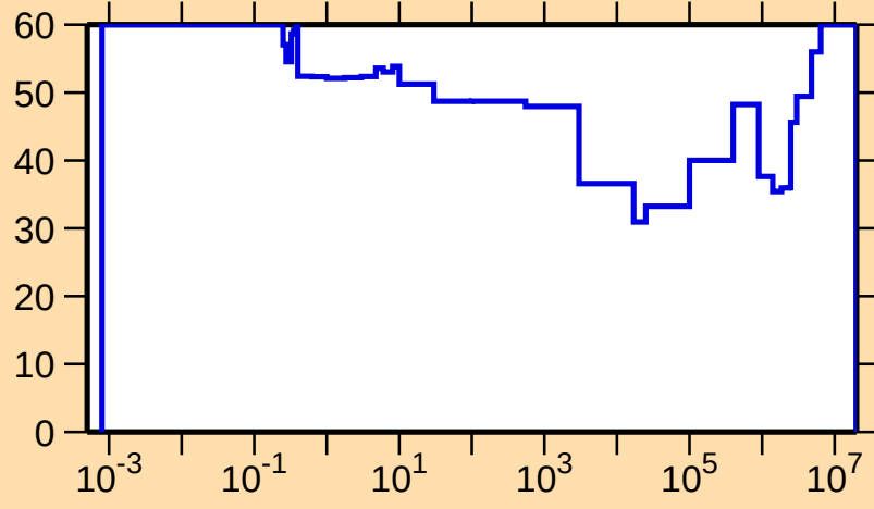
\Delta\sigma/\sigma vs. E for ^{122}\text{Cs}(n,p)
