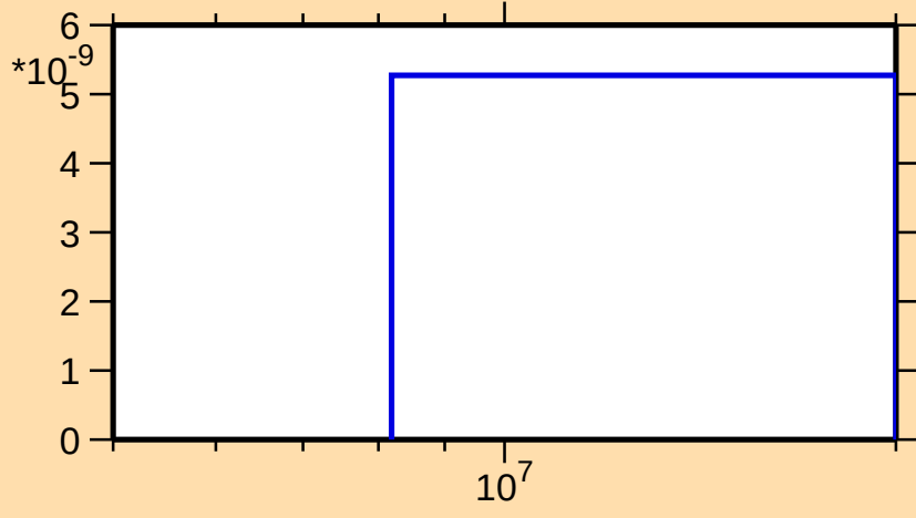
\sigma vs. E for ^{122}\text{Cs}(\text{mt117})
