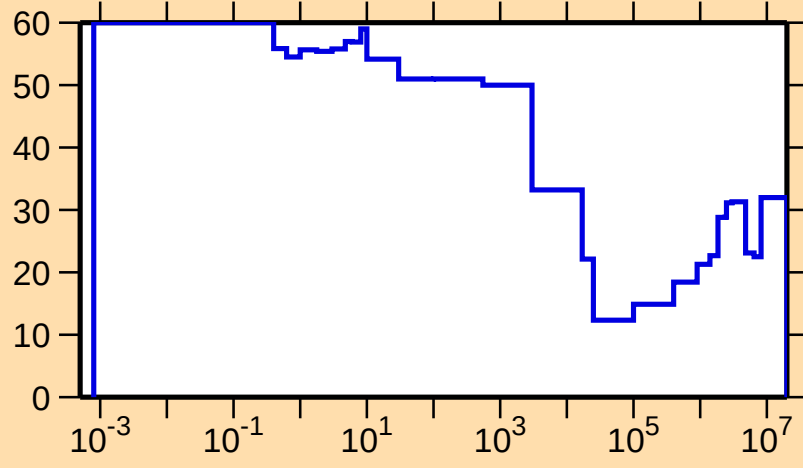
\Delta\sigma/\sigma vs. E for ^{122}\text{Cs}(n,\text{nonel.})
