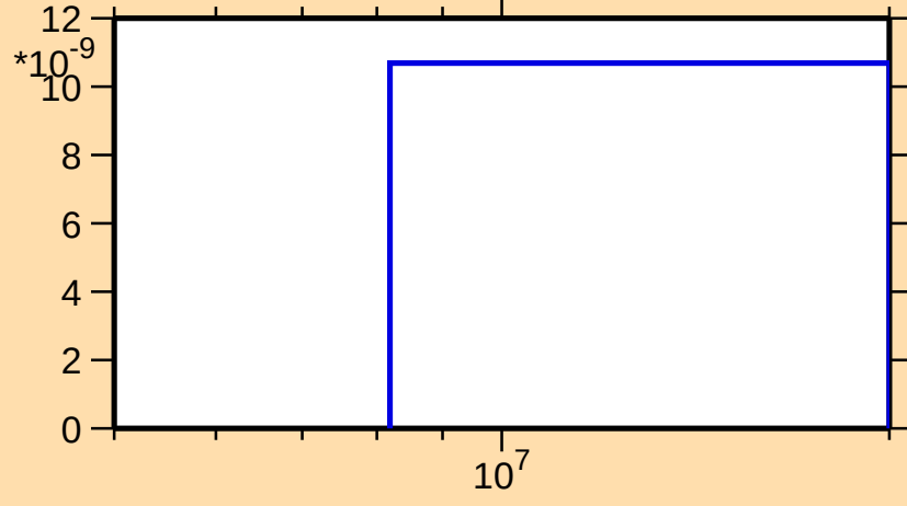
\sigma vs. E for ^{122}\text{Cs}(n,\text{pt})
