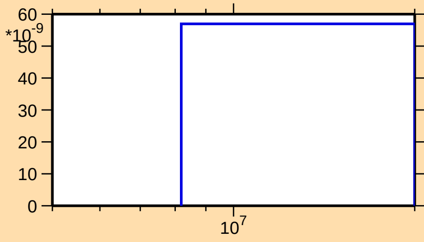
\sigma vs. E for ^{122}\text{Cs}(n,\text{pd})
