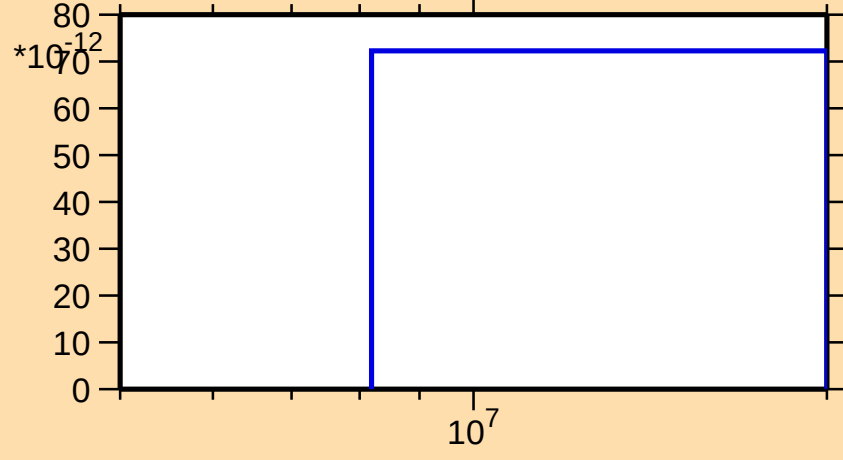
\sigma vs. E for ^{122}\text{Cs}(n,nt)
