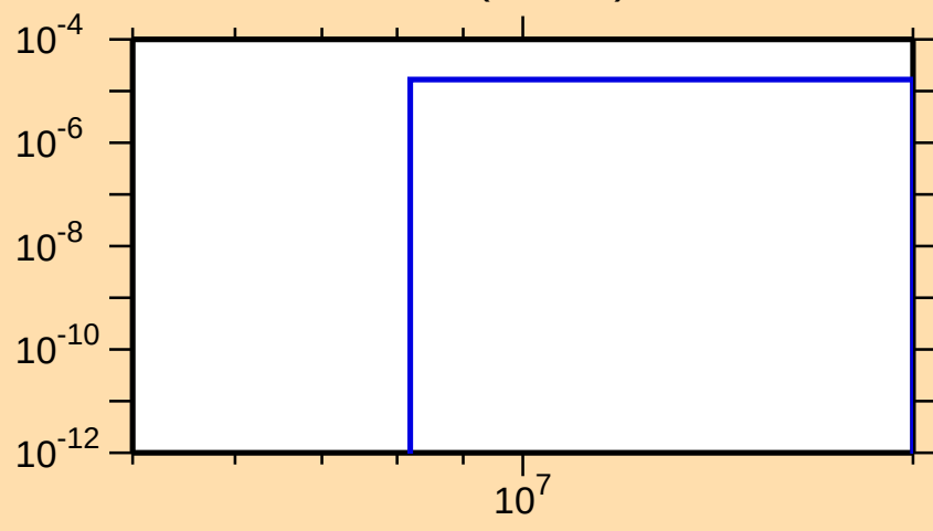
\sigma vs. E for ^{122}\text{Cs}(n,\text{He}3)
