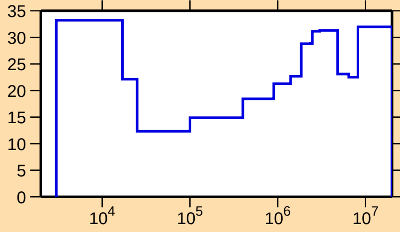
\Delta\sigma/\sigma vs. E for ^{122}\text{Cs}(n,\text{nonel.})
