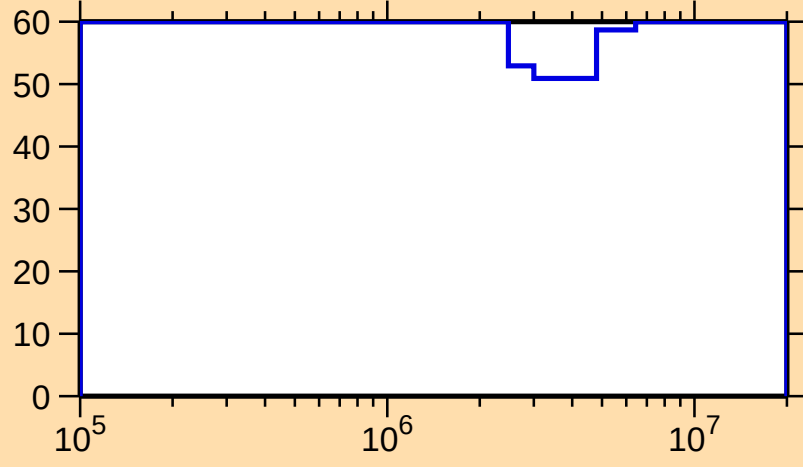
\Delta\sigma/\sigma vs. E for ^{122}\text{Cs}(n,n\text{cont.})
