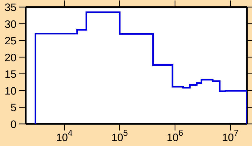
\Delta\sigma/\sigma vs. E for ^{122}\text{Cs}(n,\text{el.})
