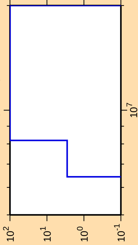
\Delta\sigma/\sigma vs. E for ^{122}\text{Cs}(n,\text{He}3)
