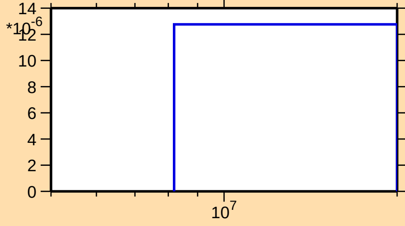
\sigma vs. E for ^{122}\text{Cs}(n,\text{nd})
