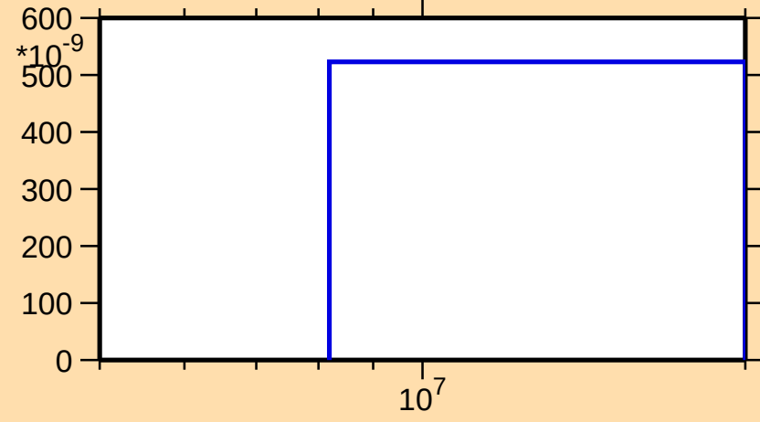
\sigma vs. E for ^{122}\text{Cs} (mt 45)
