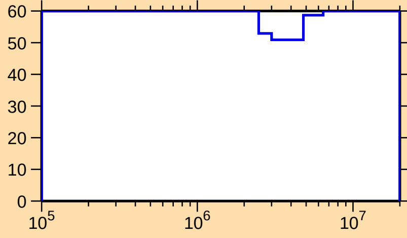
\Delta\sigma/\sigma vs. E for ^{122}\text{Cs}(n,n\text{cont.})
