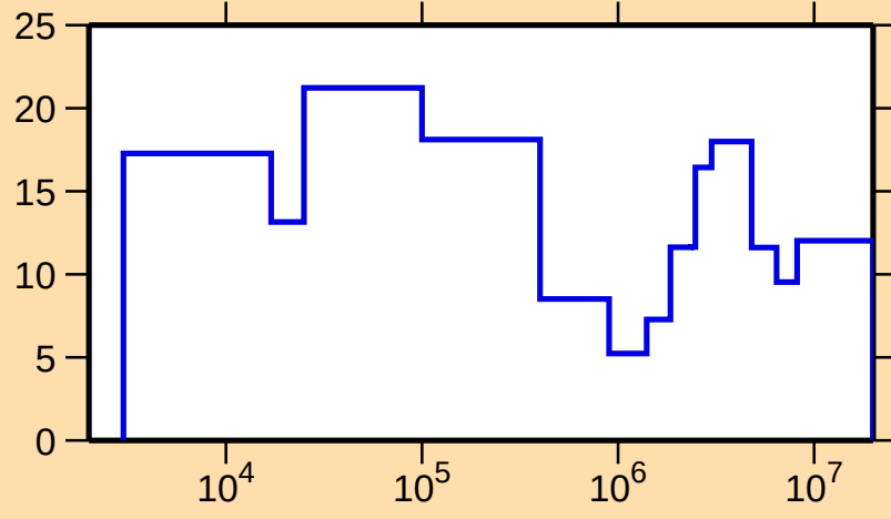
\Delta\sigma/\sigma vs. E for ^{122}\text{Cs}(n,\text{tot.})
