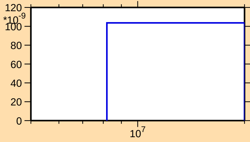
\sigma vs. E for ^{122}\text{Cs}(n,2n\alpha)
