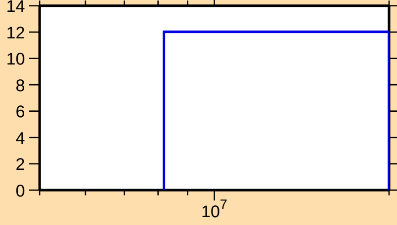
\Delta\sigma/\sigma vs. E for ^{122}\text{Cs}(n,\text{tot.})
