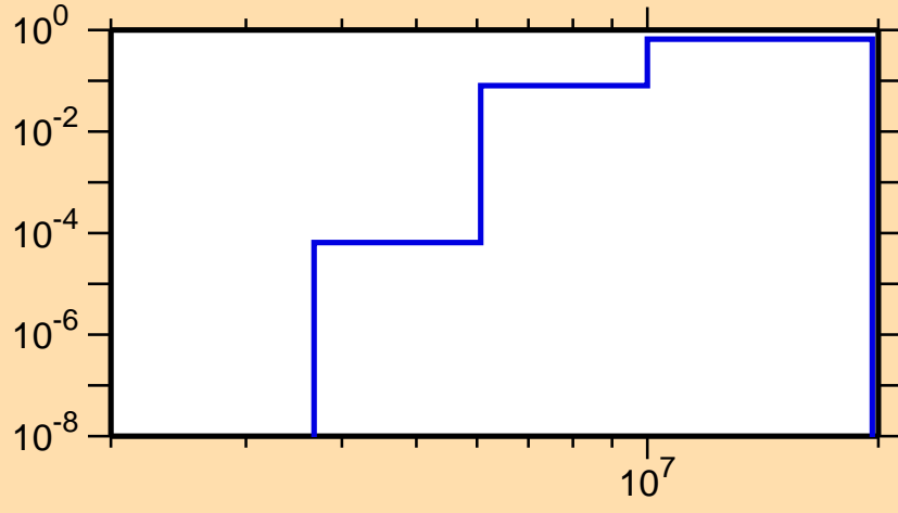
\sigma vs. E for ^{123}\text{Cs}(n,np)
