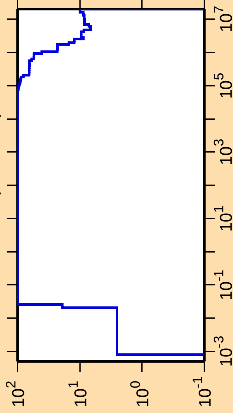
\Delta\sigma/\sigma vs. E for ^{123}\text{Cs}(n,\text{nonel.})
