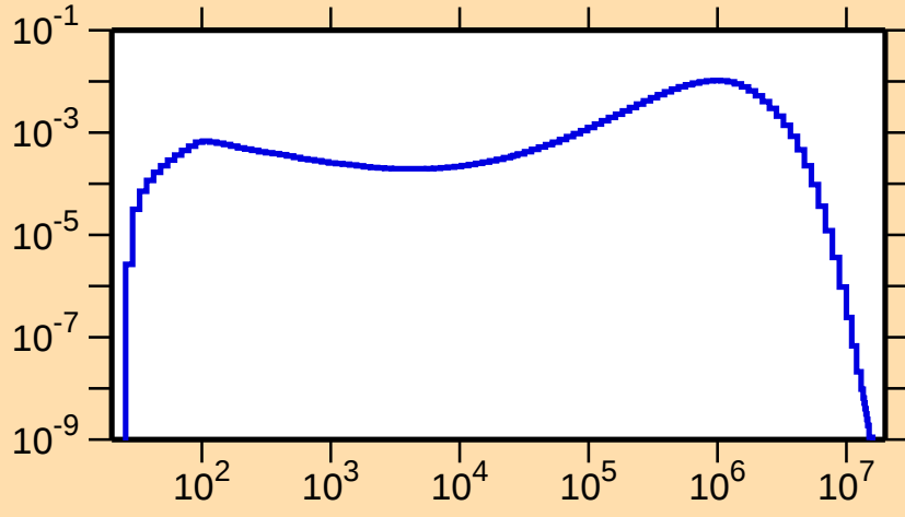
\sigma vs. E for ^{123}\text{Cs}(n,n_2)
