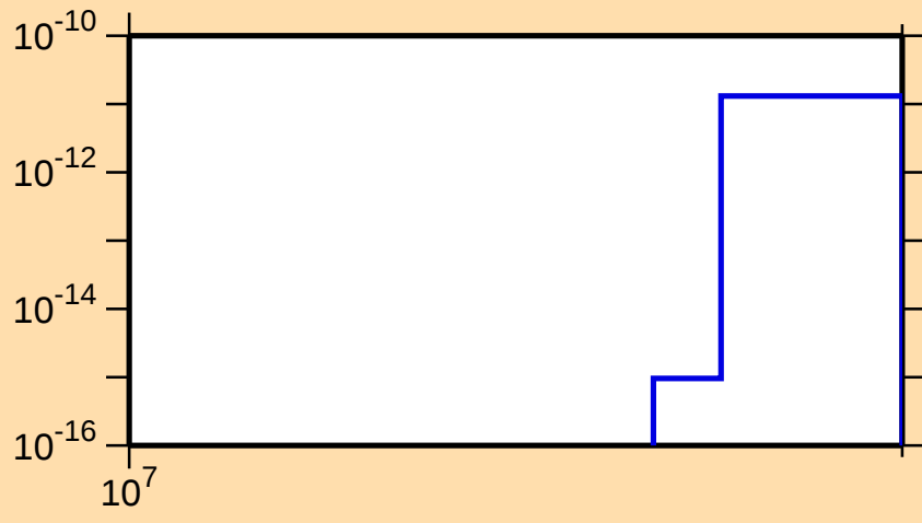
\sigma vs. E for ^{123}\text{Cs}(n,\text{pt})
