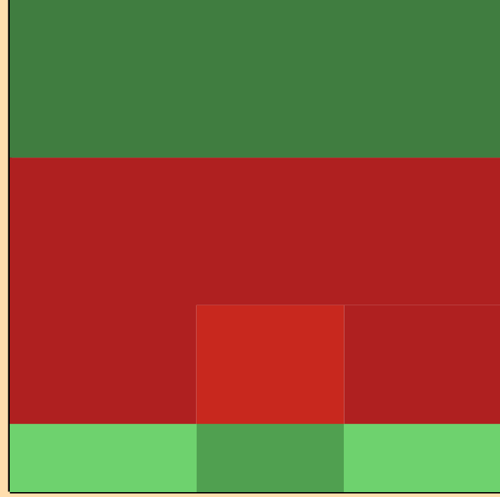
\Delta\sigma/\sigma vs. E for ^{123}\text{Cs}(n,\text{nonel.})
