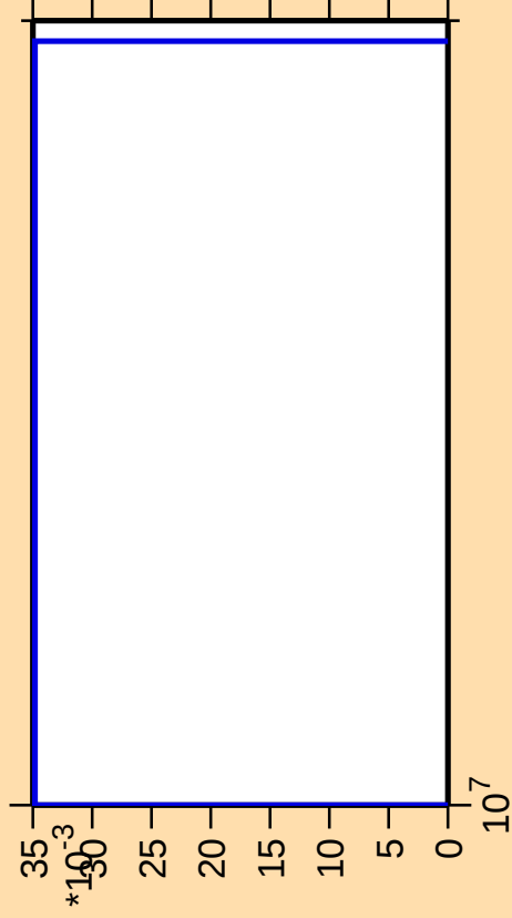
\Delta\sigma/\sigma vs. E for ^{123}\text{Cs} (mt 34)
