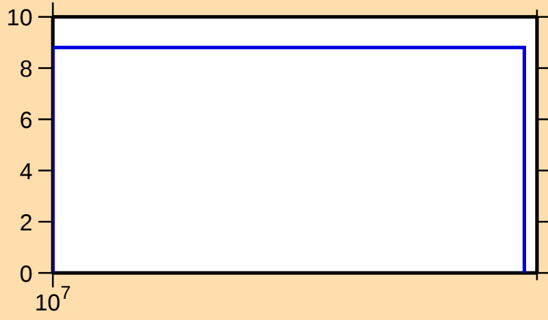
\Delta\sigma/\sigma vs. E for ^{123}\text{Cs}(n,\text{nonel.})
