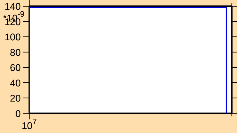
\sigma vs. E for ^{123}\text{Cs}(n,\text{nd})
