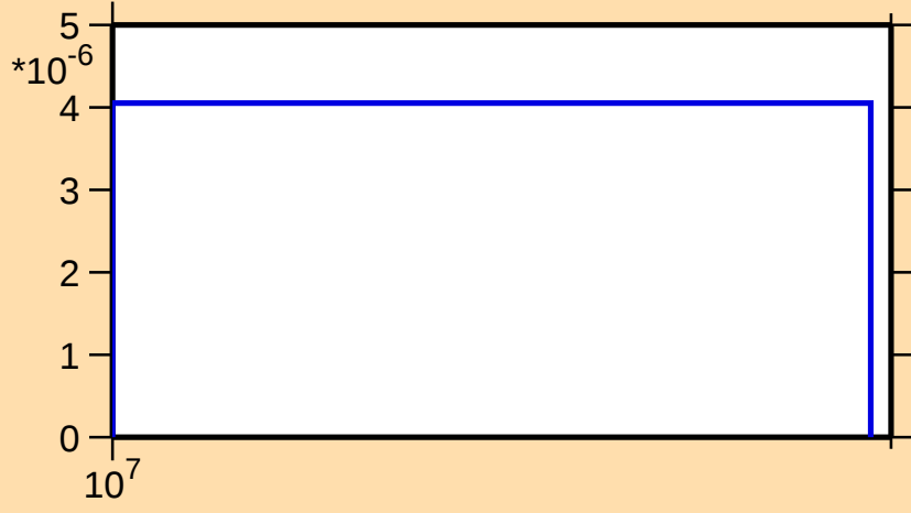
\sigma vs. E for ^{123}\text{Cs}(n,2np)
