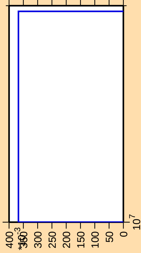
\Delta\sigma/\sigma vs. E for ^{123}\text{Cs}(n,\text{pt})
