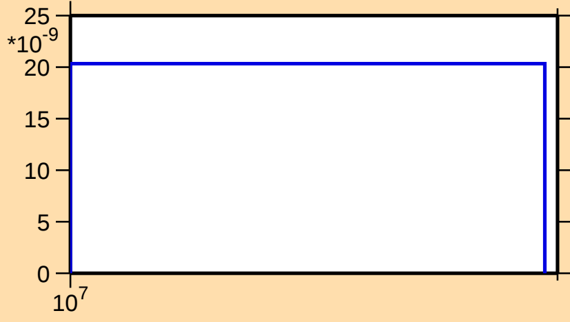
\sigma vs. E for ^{123}\text{Cs}(n,\text{pd})
