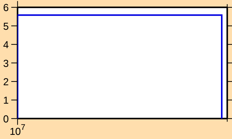
\Delta\sigma/\sigma vs. E for ^{123}\text{Cs}(n,\text{el.})
