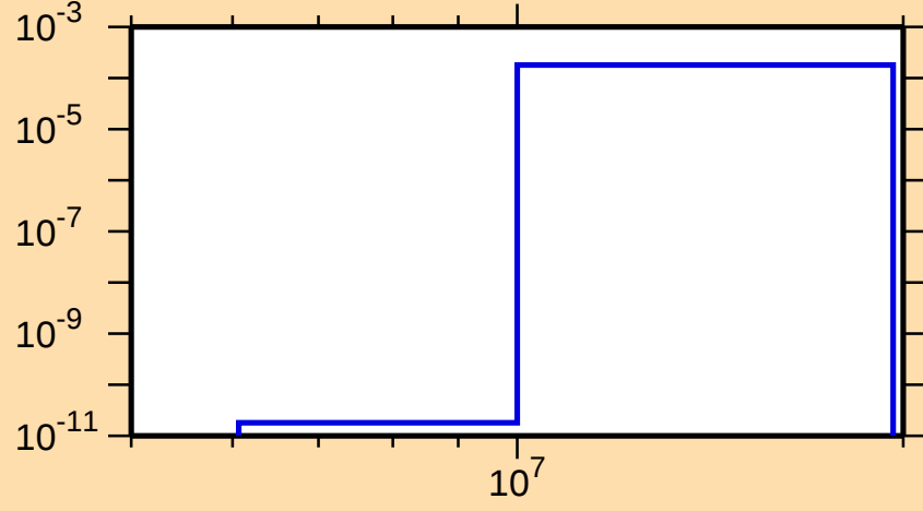
\sigma vs. E for ^{123}\text{Cs}(n,t)
