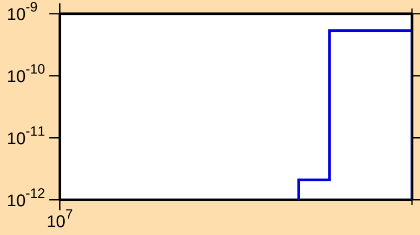
\sigma vs. E for ^{124}\text{Cs} (mt 34)
