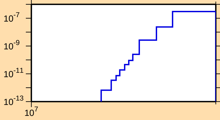
\sigma vs. E for ^{124}\text{Cs} (mt 45)
