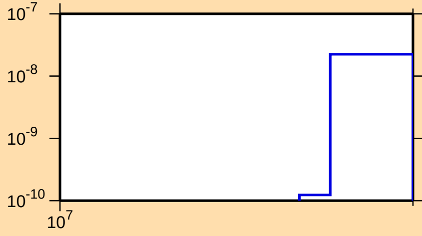
\sigma vs. E for ^{124}\text{Cs}(n,\text{pt})
