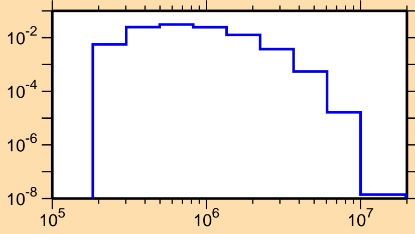
\sigma vs. E for ^{124}\text{Cs}(n,n_3)
