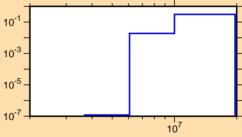
\sigma vs. E for ^{124}\text{Cs}(n,np)
