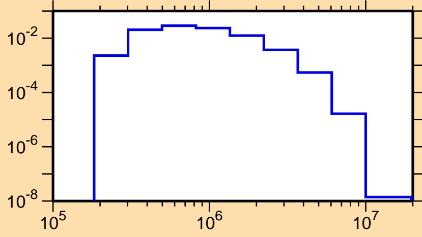
\sigma vs. E for ^{124}\text{Cs}(n,n_4)
