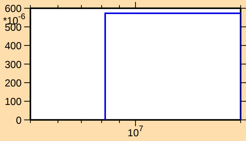
\sigma vs. E for ^{124}\text{Cs}(n,2np)
