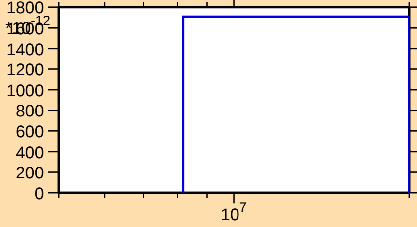
\sigma vs. E for ^{124}\text{Cs}(n,\text{pd})
