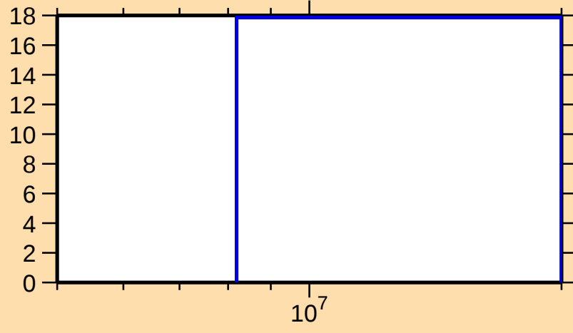
\Delta\sigma/\sigma vs. E for ^{124}\text{Cs}(n,\text{nonel.})
