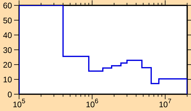
\Delta\sigma/\sigma vs. E for ^{124}\text{Cs}(n,\text{tot.})
