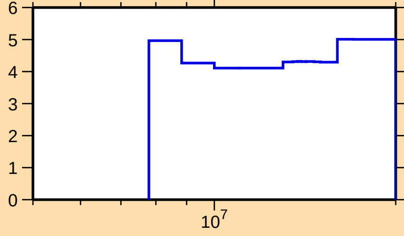
\Delta\sigma/\sigma vs. E for ^{124}\text{Cs}(n,\text{nonel.})
