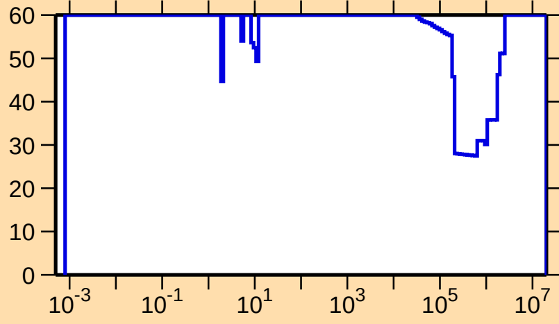
\Delta\sigma/\sigma vs. E for ^{124}\text{Cs}(n,\gamma)
