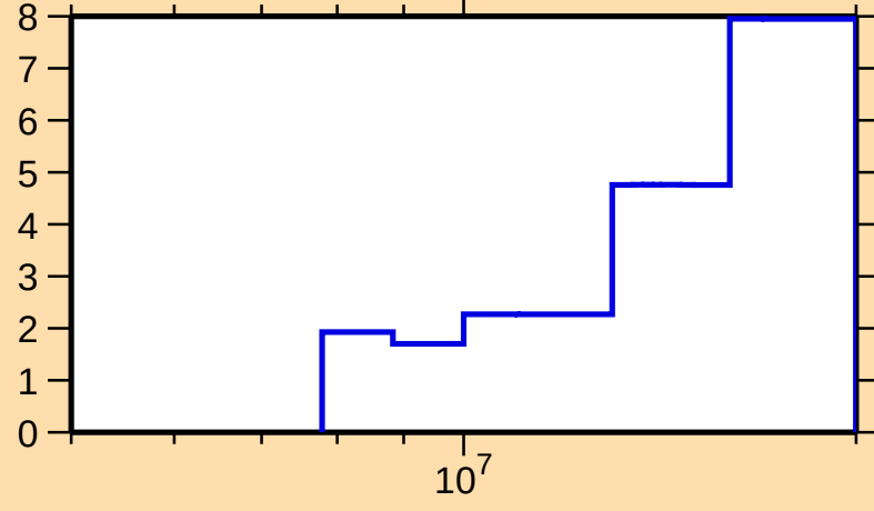
\Delta\sigma/\sigma vs. E for ^{124}\text{Cs}(n,\text{tot.})
