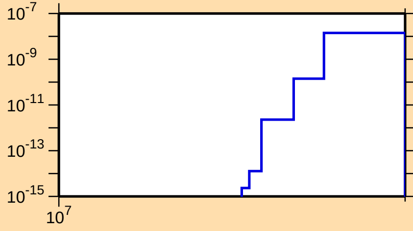
\sigma vs. E for ^{124}\text{Cs}(n,\text{pt})
