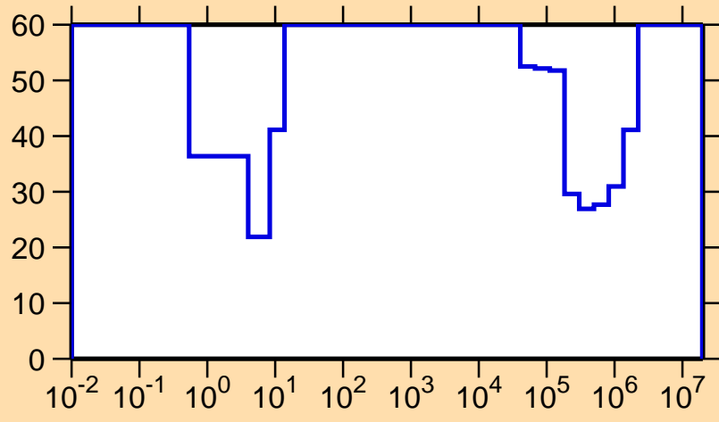
\Delta\sigma/\sigma vs. E for ^{124}\text{Cs}(n,\gamma)
