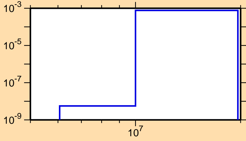
\sigma vs. E for ^{124}\text{Cs}(n,t)
