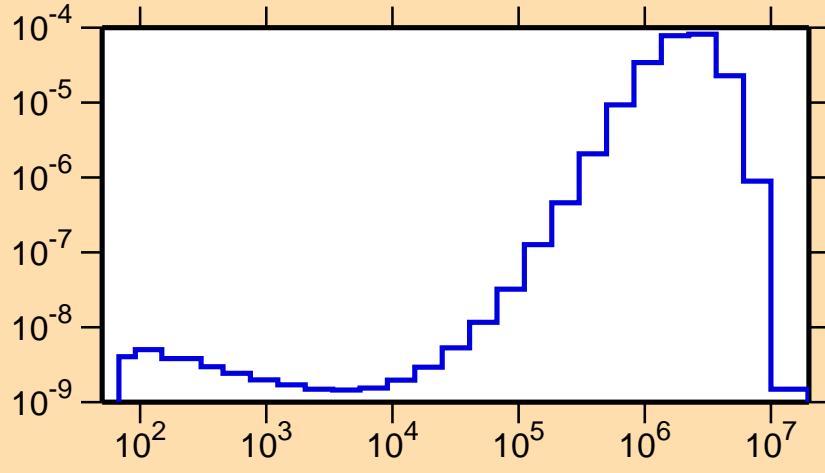
\sigma vs. E for ^{124}\text{Cs}(n,n_2)
