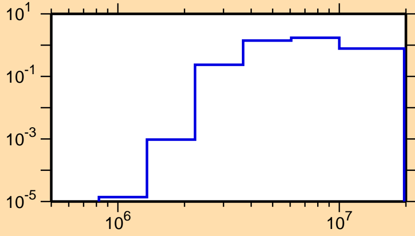
\sigma vs. E for ^{125}\text{Cs}(n,n\text{cont.})
