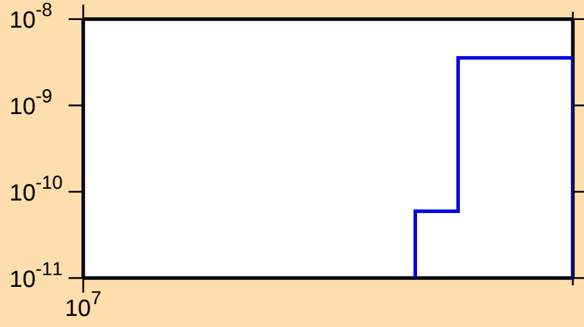
\sigma vs. E for ^{126}\text{Cs}(n,\text{pd})
