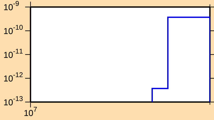
\sigma vs. E for ^{126}\text{Cs}(n,\text{pt})
