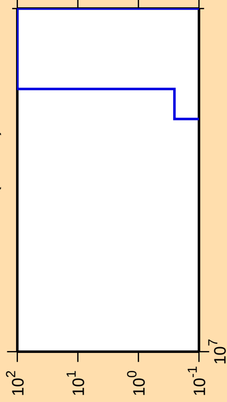
\Delta\sigma/\sigma vs. E for ^{126}\text{Cs} (mt 34)
