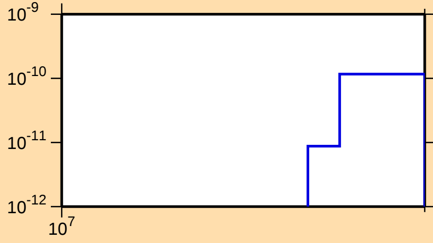
\sigma vs. E for ^{126}\text{Cs}(\text{mt117})
