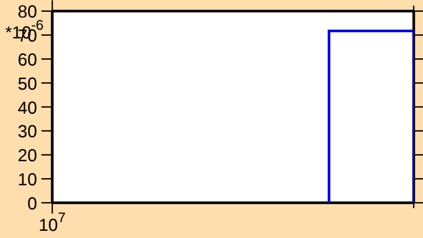
\sigma vs. E for ^{126}\text{Cs}(n,3n)
