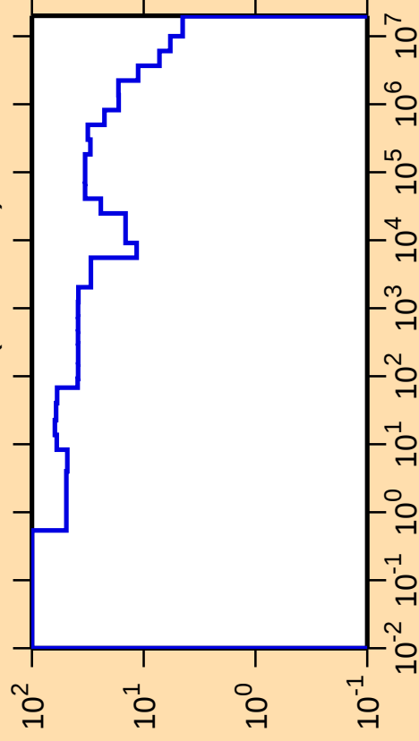
\Delta\sigma/\sigma vs. E for ^{126}\text{Cs}(n,\text{nonel.})
