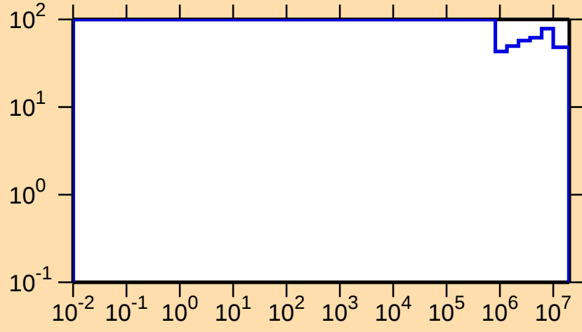
\Delta\sigma/\sigma vs. E for ^{126}\text{Cs}(n,p)
