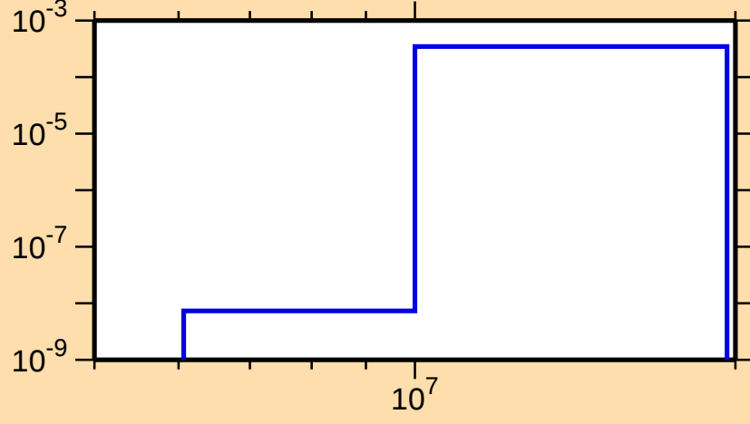
\sigma vs. E for ^{126}\text{Cs}(n,t)
