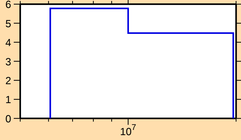
\Delta\sigma/\sigma vs. E for ^{126}\text{Cs}(n,\text{nonel.})
