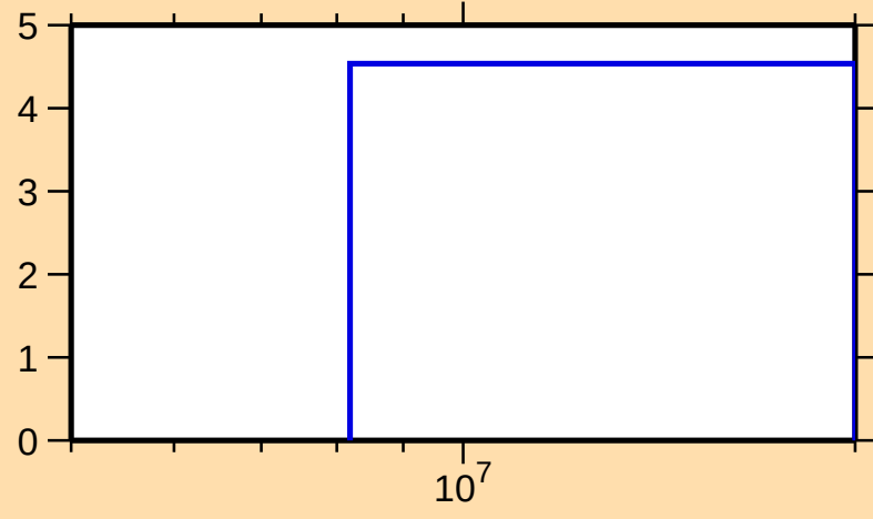
\Delta\sigma/\sigma vs. E for ^{126}\text{Cs}(n,\text{nonel.})
