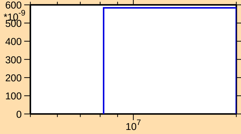
\sigma vs. E for ^{126}\text{Cs}(n,3n)
