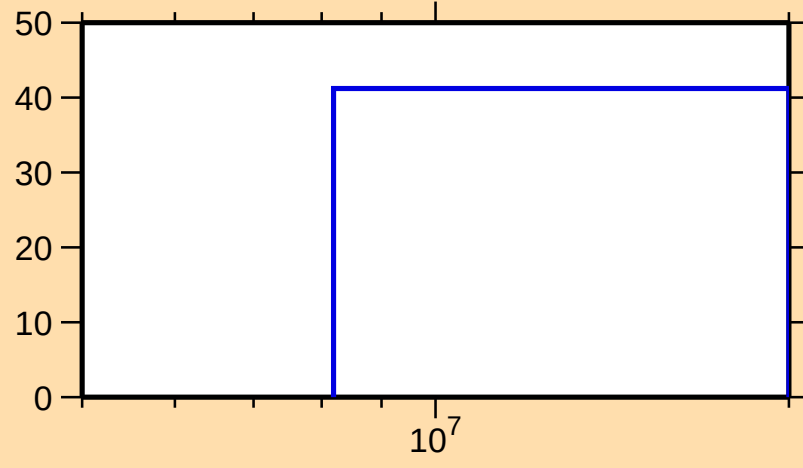
\Delta\sigma/\sigma vs. E for ^{126}\text{Cs}(n,\text{inel.})
