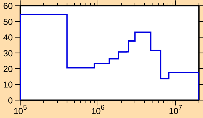
\Delta\sigma/\sigma vs. E for ^{126}\text{Cs}(n,\text{el.})
