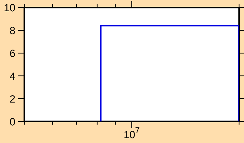
\Delta\sigma/\sigma vs. E for ^{126}\text{Cs}(n,\text{tot.})
