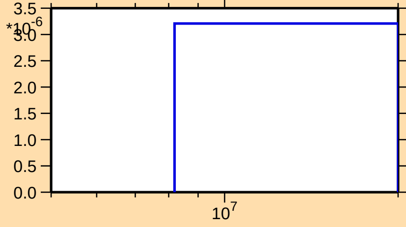
\sigma vs. E for ^{126}\text{Cs}(n,\text{nd})
