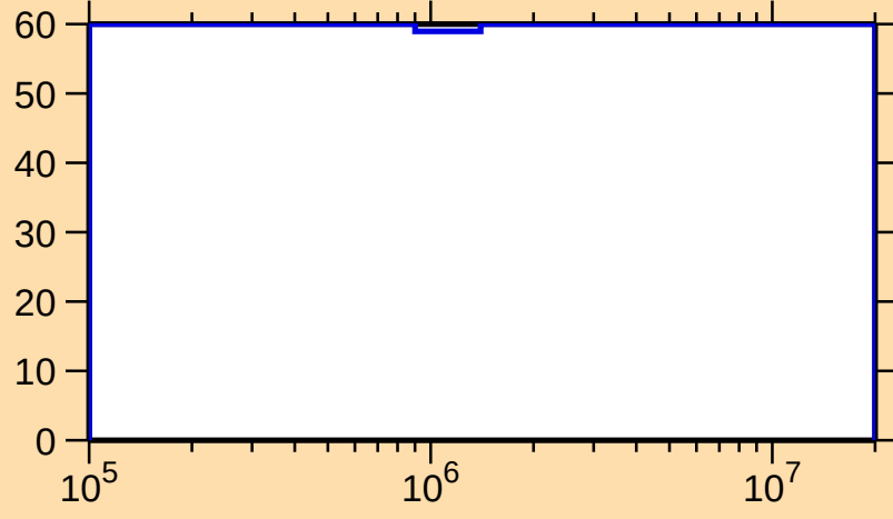
\Delta\sigma/\sigma vs. E for ^{126}\text{Cs}(n,n_1)
