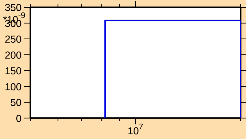
\sigma vs. E for ^{126}\text{Cs}(n,\text{He}3)
