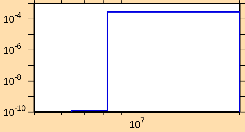
\sigma vs. E for ^{126}\text{Cs}(n,t)
