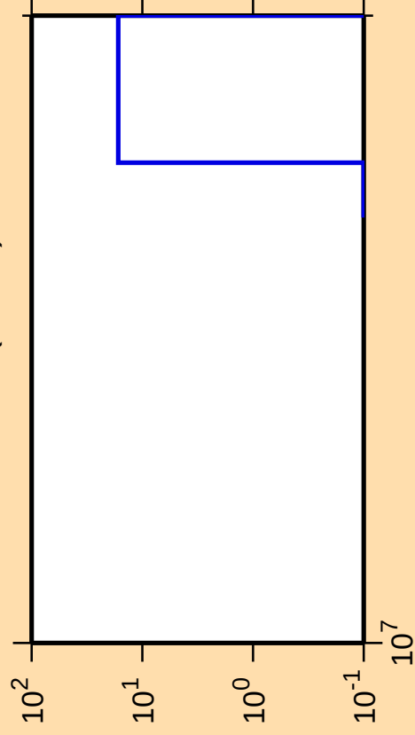
\Delta\sigma/\sigma vs. E for ^{128}\text{Cs} (mt 34)
