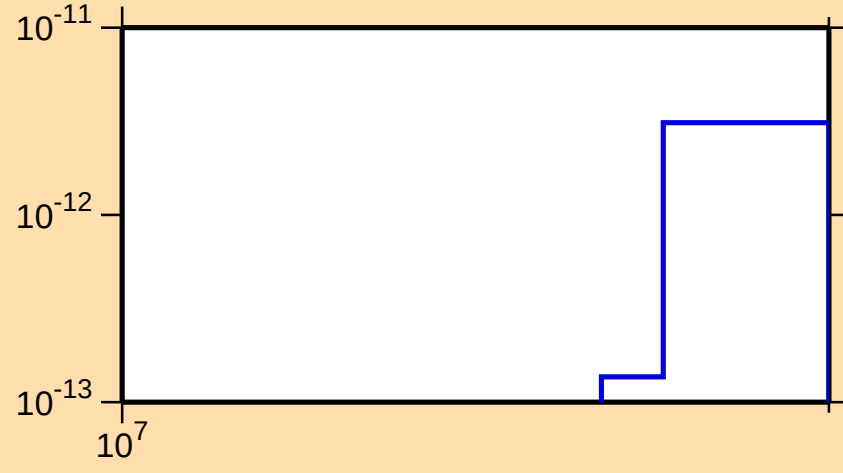
\sigma vs. E for ^{128}\text{Cs}(\text{mt117})
