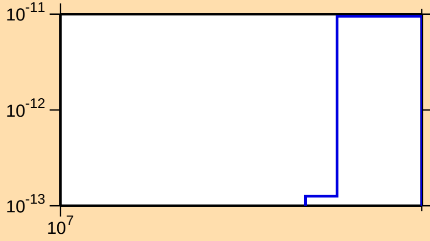
\sigma vs. E for ^{128}\text{Cs} (mt 45)
