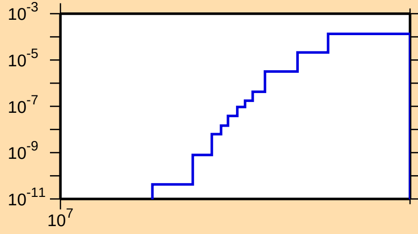
\sigma vs. E for ^{128}\text{Cs}(n,nd)
