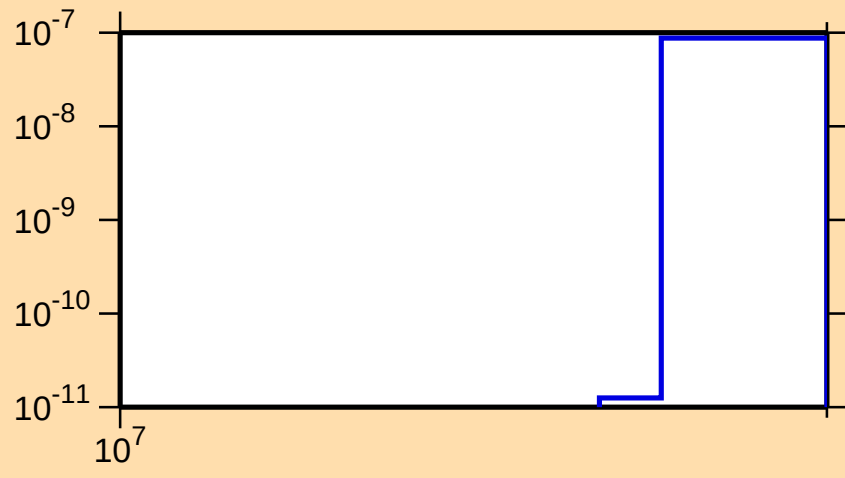
\sigma vs. E for ^{128}\text{Cs}(n,nt)
