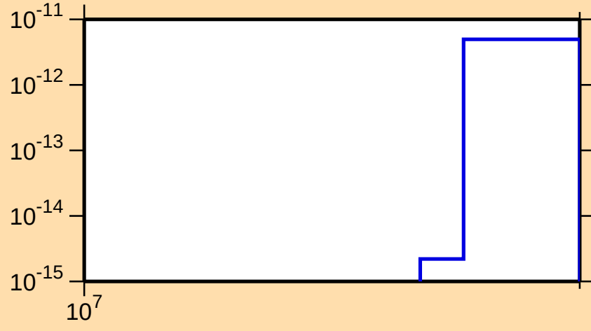
\sigma vs. E for ^{128}\text{Cs}(n,\text{pt})
