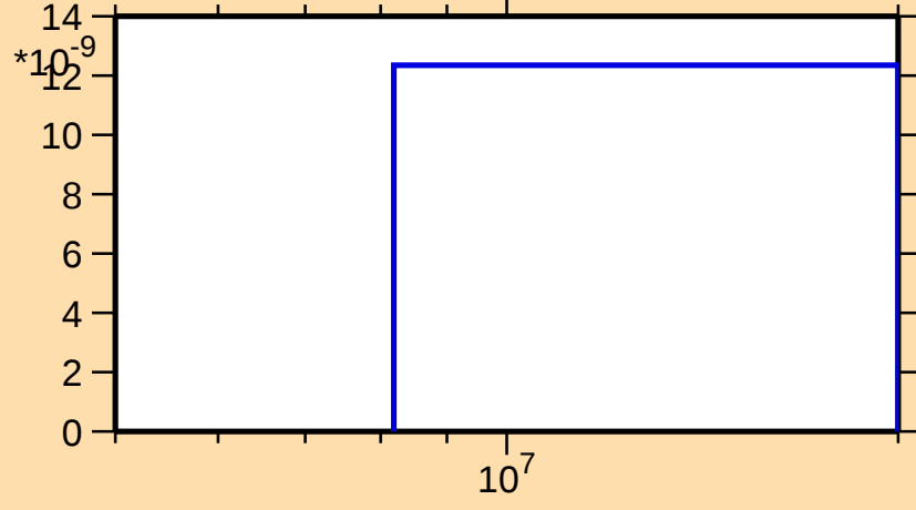
\sigma vs. E for ^{128}\text{Cs}(n,2n\alpha)
