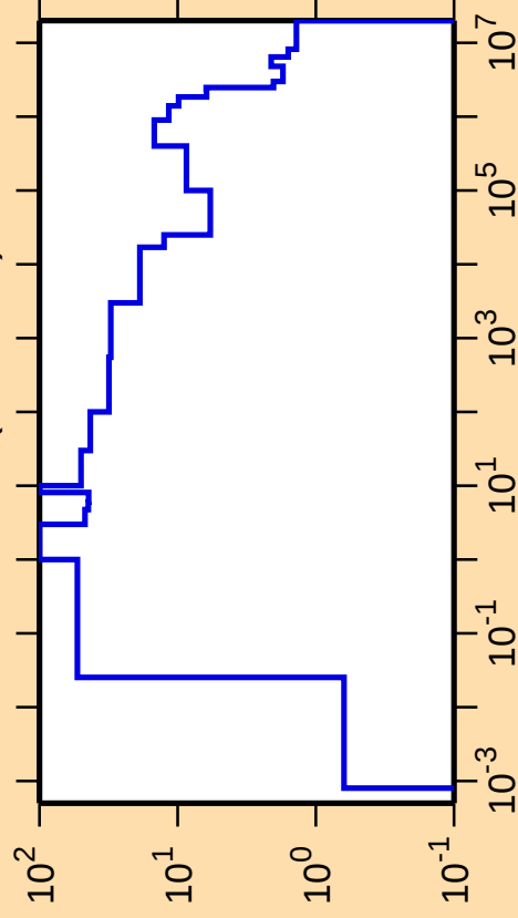
\Delta\sigma/\sigma vs. E for ^{128}\text{Cs}(n,\text{nonel.})
