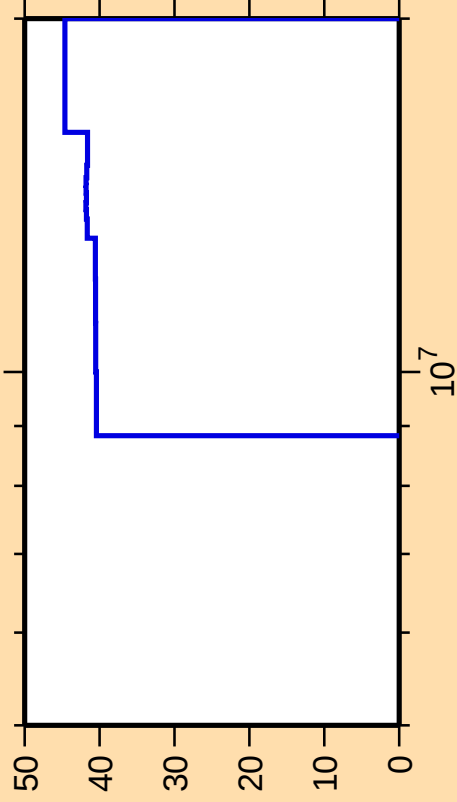
\Delta\sigma/\sigma vs. E for ^{129}\text{Cs}(n,n_1)
