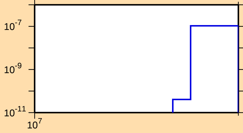
\sigma vs. E for ^{129}\text{Cs}(n,nt)
