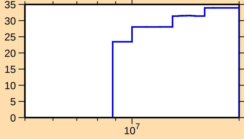
\Delta\sigma/\sigma vs. E for ^{129}\text{Cs}(n,\text{inel.})
