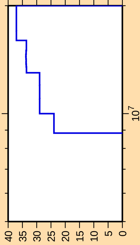
\Delta\sigma/\sigma vs. E for ^{129}\text{Cs}(n,n\text{cont.})
