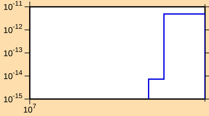
\sigma vs. E for ^{129}\text{Cs}(n,\text{pd})
