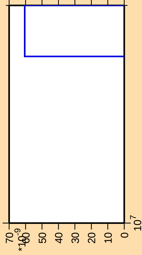
\Delta\sigma/\sigma vs. E for ^{129}\text{Cs} (mt 11)
