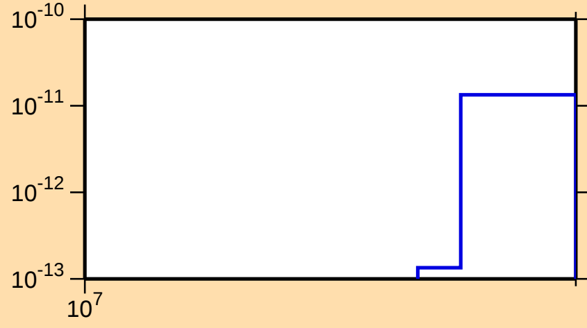
\sigma vs. E for ^{129}\text{Cs} (mt 45)
