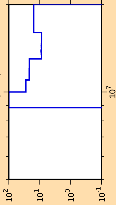
\Delta\sigma/\sigma vs. E for ^{129}\text{Cs}(n,2n)
