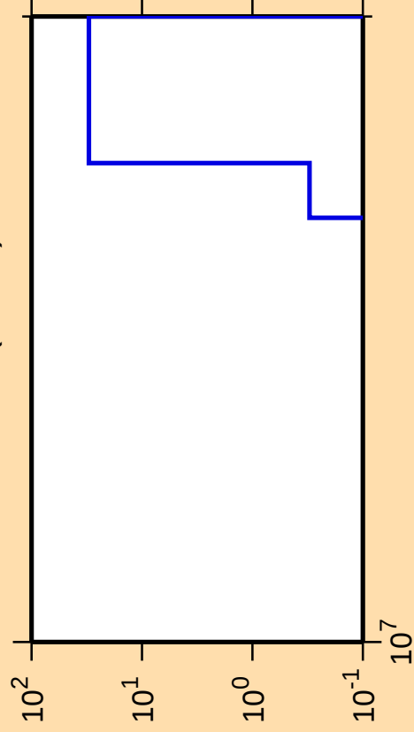
\Delta\sigma/\sigma vs. E for ^{129}\text{Cs} (mt 45)
