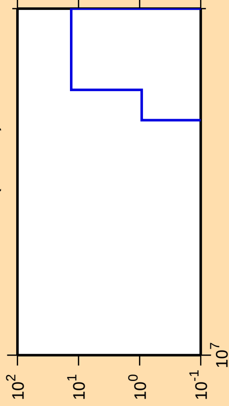
\Delta\sigma/\sigma vs. E for ^{129}\text{Cs}(\text{mt117})
