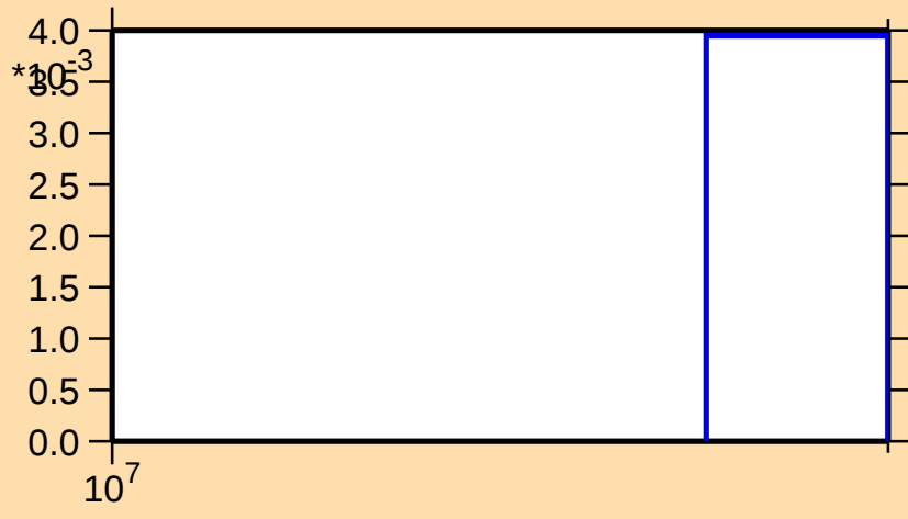
\sigma vs. E for ^{129}\text{Cs}(n,3n)
