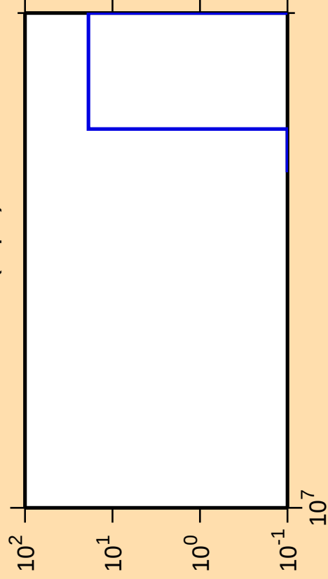
\Delta\sigma/\sigma vs. E for ^{129}\text{Cs}(n,\text{pd})
