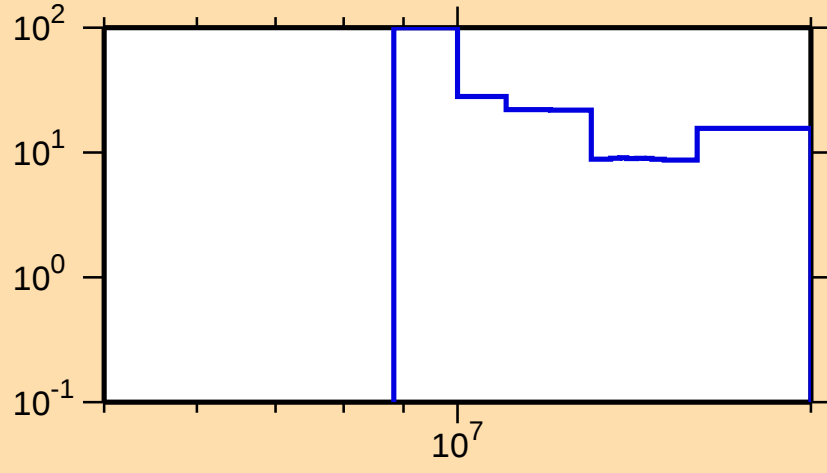
\Delta\sigma/\sigma vs. E for ^{129}\text{Cs}(n,2n)
