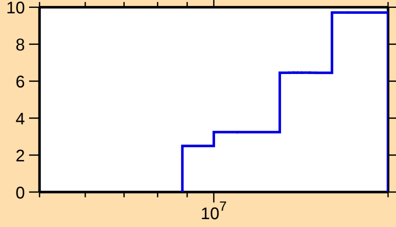
\Delta\sigma/\sigma vs. E for ^{129}\text{Cs}(n,\text{tot.})
