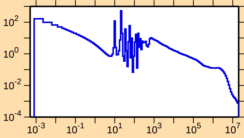
\sigma vs. E for ^{129}\text{Cs}(n,\gamma)
