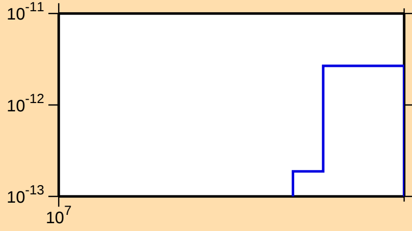
\sigma vs. E for ^{129}\text{Cs}(\text{mt117})
