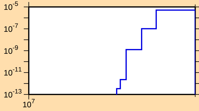
\sigma vs. E for ^{129}\text{Cs}(n,\text{nd})
