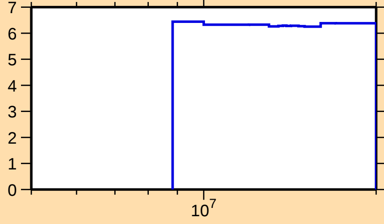
\Delta\sigma/\sigma vs. E for ^{129}\text{Cs}(n,\text{nonel.})
