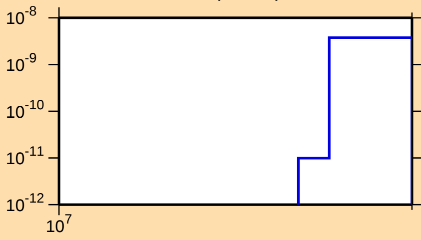
\sigma vs. E for ^{129}\text{Cs}(n,2n\alpha)
