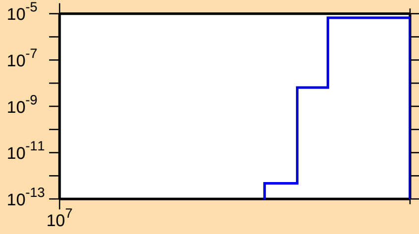
\sigma vs. E for ^{129}\text{Cs}(n,2np)
