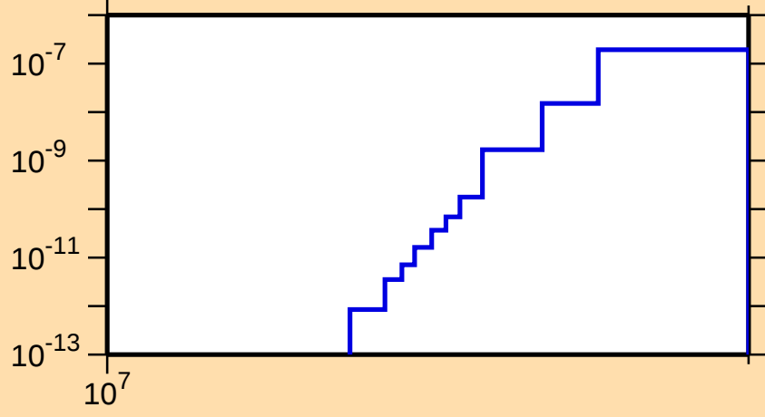
\sigma vs. E for ^{129}\text{Cs}(n,\text{He}3)
