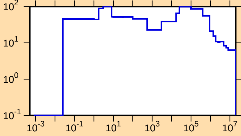
\Delta\sigma/\sigma vs. E for ^{129}\text{Cs}(n,\text{nonel.})
