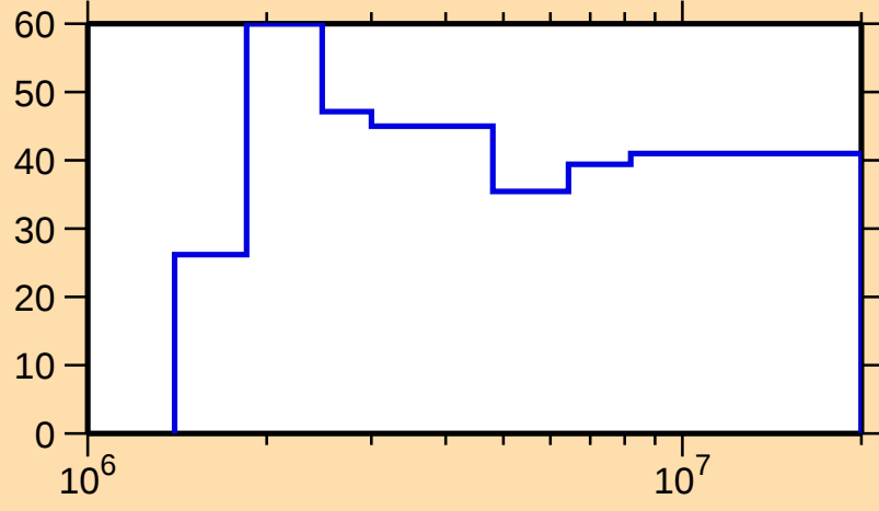
\Delta\sigma/\sigma vs. E for ^{129}\text{Cs}(n,n_1)
