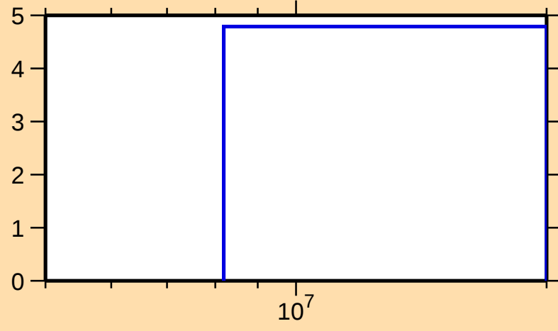
\Delta\sigma/\sigma vs. E for ^{129}\text{Cs}(n,\text{tot.})
