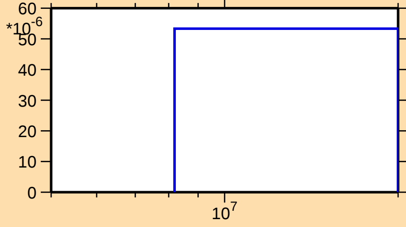
\sigma vs. E for ^{129}\text{Cs}(n,t)
