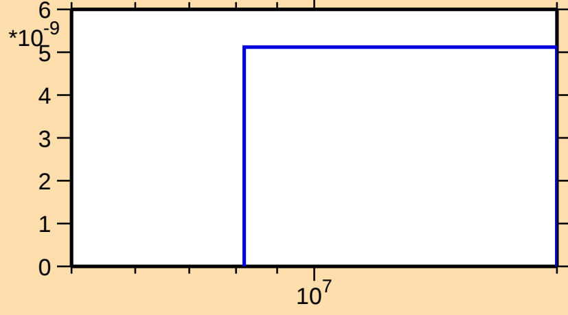
\sigma vs. E for ^{129}\text{Cs}(n,p\alpha)
