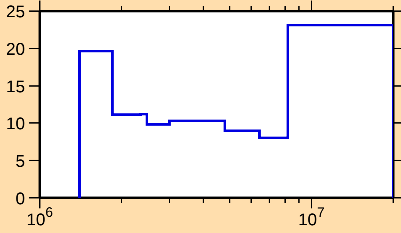
\Delta\sigma/\sigma vs. E for ^{129}\text{Cs}(n,\text{inel.})
