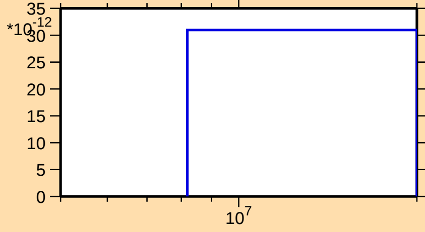
\sigma vs. E for ^{129}\text{Cs}(n,2n\alpha)
