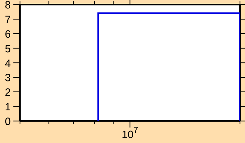
\Delta\sigma/\sigma vs. E for ^{129}\text{Cs}(n,\text{el.})
