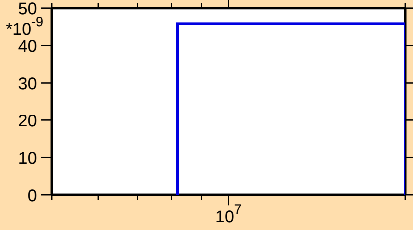
\sigma vs. E for ^{129}\text{Cs}(n,\text{nd})
