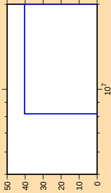
\Delta\sigma/\sigma vs. E for ^{129}\text{Cs}(n,p)
