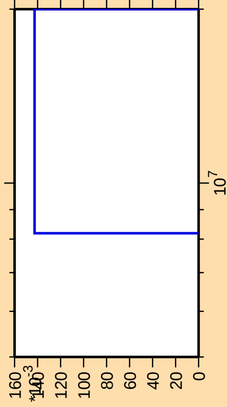
\Delta\sigma/\sigma vs. E for ^{129}\text{Cs}(\text{mt117})
