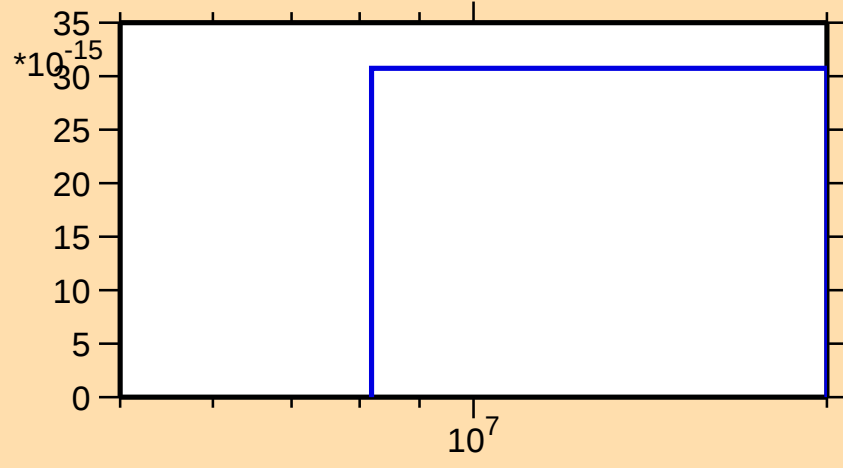
\sigma vs. E for ^{129}\text{Cs}(\text{mt117})
