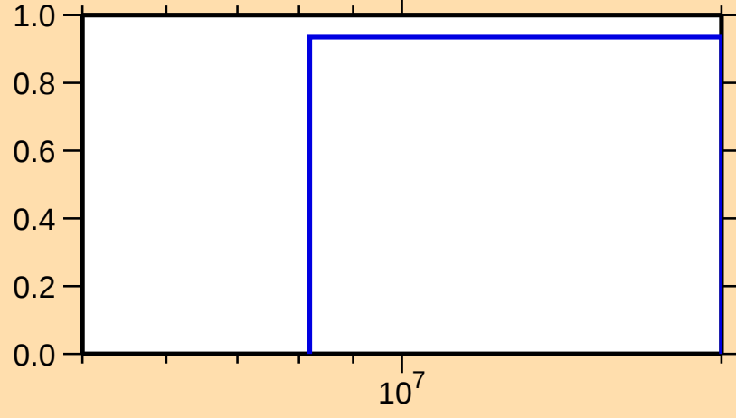
\sigma vs. E for ^{129}\text{Cs}(n,2n)
