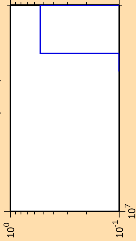
\Delta\sigma/\sigma vs. E for ^{130}\text{Cs} (mt 45)
