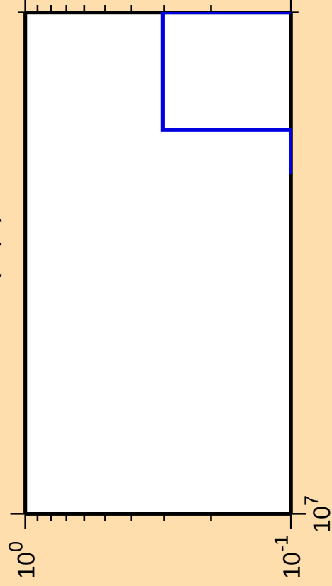
\Delta\sigma/\sigma vs. E for ^{130}\text{Cs}(n,\text{pt})
