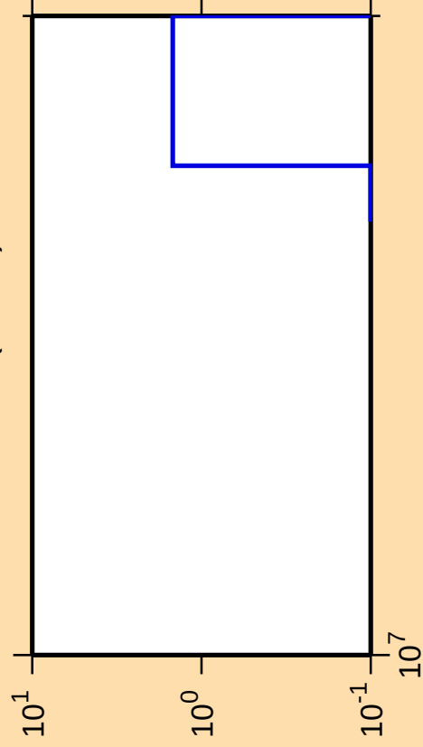
\Delta\sigma/\sigma vs. E for ^{130}\text{Cs} (mt 34)
