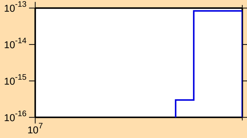
\sigma vs. E for ^{130}\text{Cs} (mt 45)
