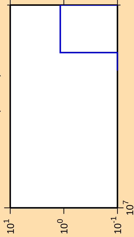
\Delta\sigma/\sigma vs. E for ^{130}\text{Cs}(\text{mt117})
