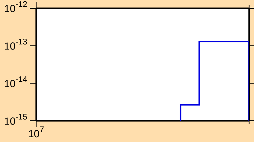
\sigma vs. E for ^{130}\text{Cs}(\text{mt117})
