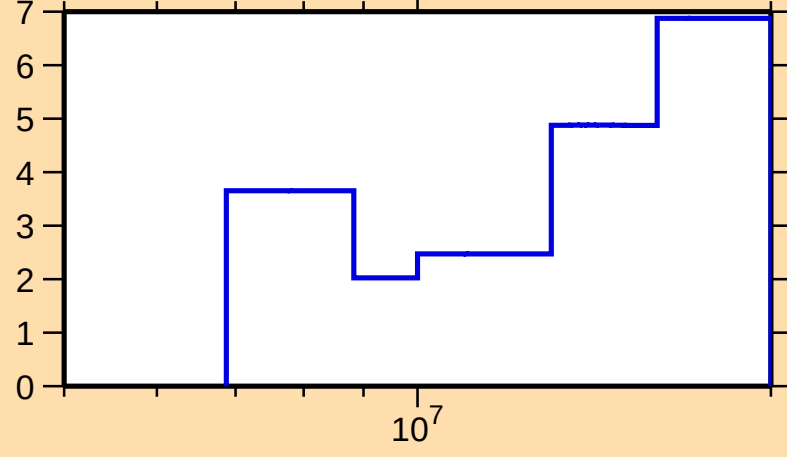
\Delta\sigma/\sigma vs. E for ^{130}\text{Cs}(n,\text{tot.})
