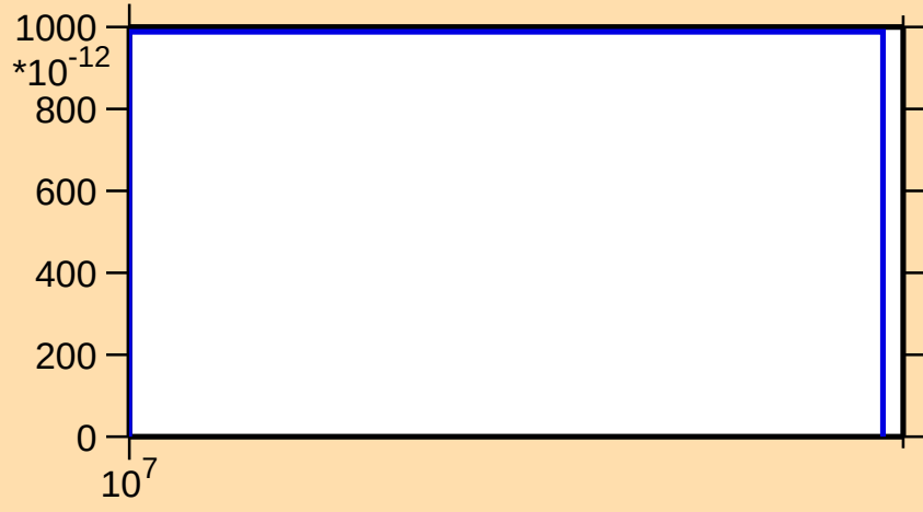
\sigma vs. E for ^{130}\text{Cs}(n,\text{nt})
