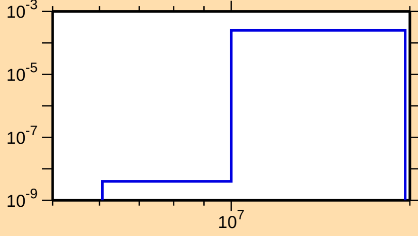
\sigma vs. E for ^{130}\text{Cs}(n,t)
