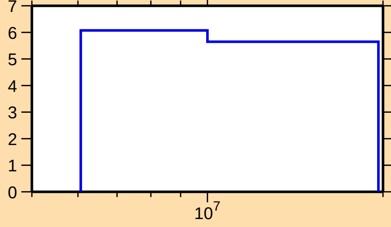
\Delta\sigma/\sigma vs. E for ^{130}\text{Cs}(n,\text{nonel.})
