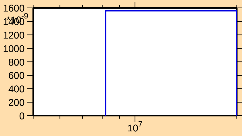
\sigma vs. E for ^{130}\text{Cs}(n,\text{nd})
