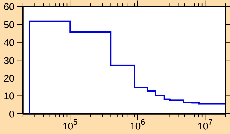
\Delta\sigma/\sigma vs. E for ^{130}\text{Cs}(n,\text{nonel.})
