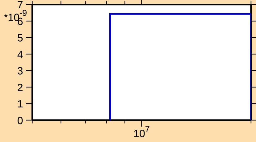
\sigma vs. E for ^{130}\text{Cs}(n,\text{He}3)
