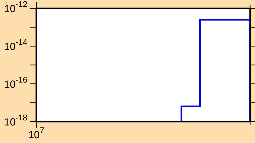
\sigma vs. E for ^{130}\text{Cs} (mt 34)
