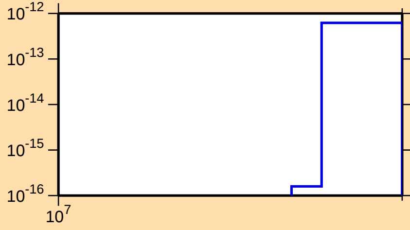
\sigma vs. E for ^{130}\text{Cs}(n,\text{pd})
