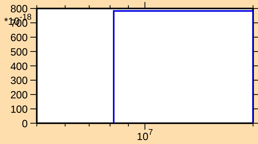
\sigma vs. E for ^{130}\text{Cs}(\text{mt } 45)
