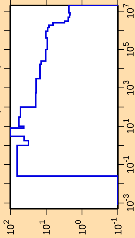
\Delta\sigma/\sigma vs. E for ^{130}\text{Cs}(n,\text{nonel.})
