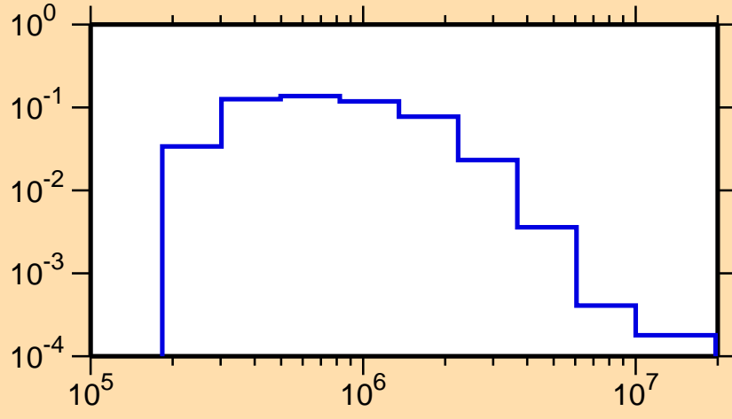
\sigma vs. E for ^{131}\text{Cs}(n,n_4)
