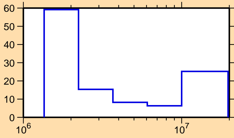
\Delta\sigma/\sigma vs. E for ^{131}\text{Cs}(n,n\text{cont.})
