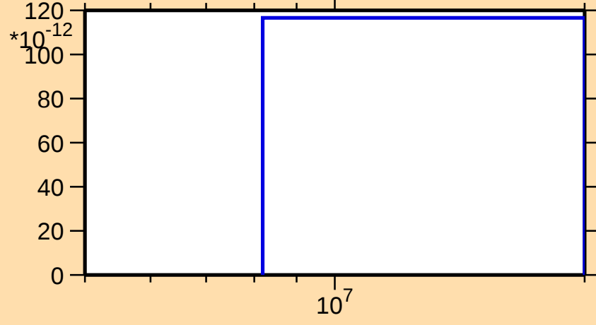
\sigma vs. E for ^{131}\text{Cs}(n,p\alpha)
