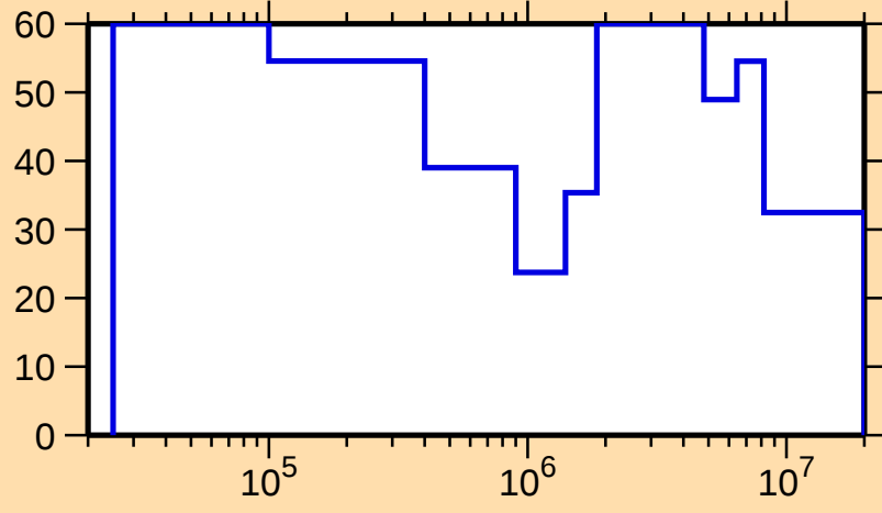
\Delta\sigma/\sigma vs. E for ^{131}\text{Cs}(n,n_1)
