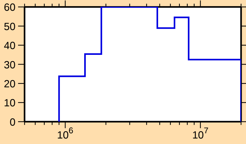
\Delta\sigma/\sigma vs. E for ^{131}\text{Cs}(n,n_1)
