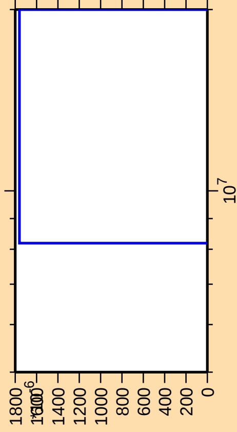
\Delta\sigma/\sigma vs. E for ^{131}\text{Cs}(n,\text{pd})
