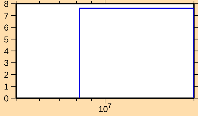
\Delta\sigma/\sigma vs. E for ^{131}\text{Cs}(n,\text{el.})
