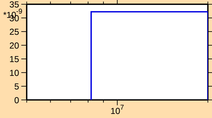
\sigma vs. E for ^{131}\text{Cs}(n,\text{nd})
