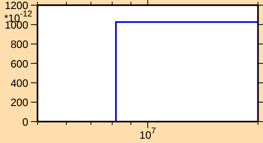
\sigma vs. E for ^{131}\text{Cs}(n,nt)
