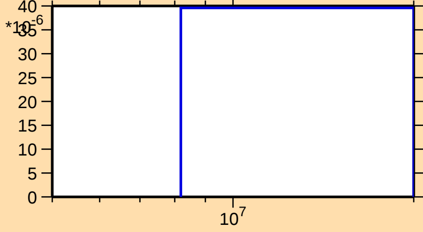
\sigma vs. E for ^{131}\text{Cs}(n,t)
