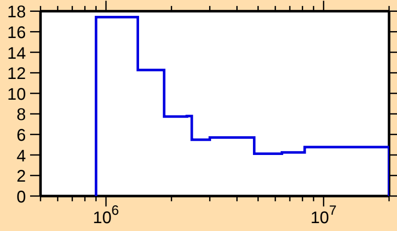
\Delta\sigma/\sigma vs. E for ^{131}\text{Cs}(n,\text{nonel.})
