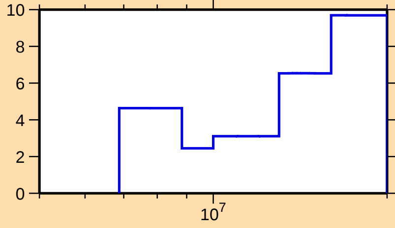
\Delta\sigma/\sigma vs. E for ^{132}\text{Cs}(n,\text{tot.})
