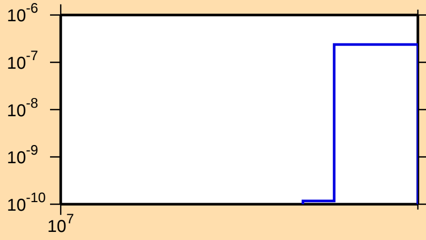
\sigma vs. E for ^{132}\text{Cs}(n,nt)
