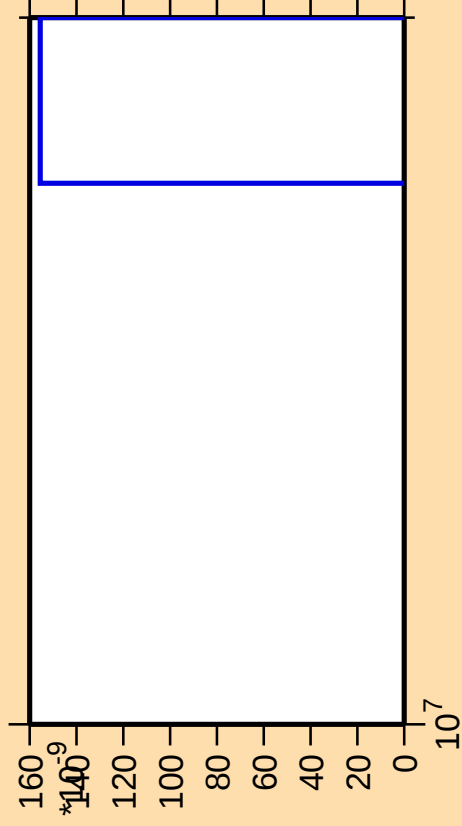
\Delta\sigma/\sigma vs. E for ^{132}\text{Cs} (mt 11)
