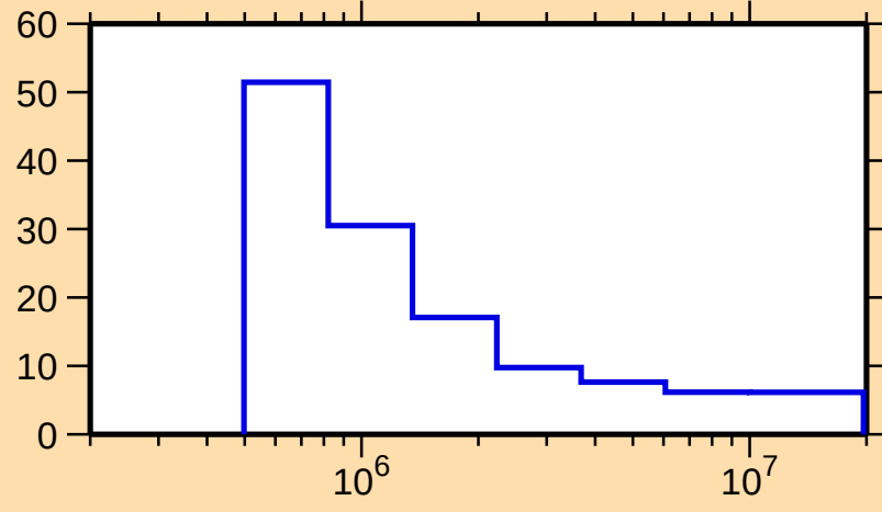
\Delta\sigma/\sigma vs. E for ^{132}\text{Cs}(n,\text{nonel.})
