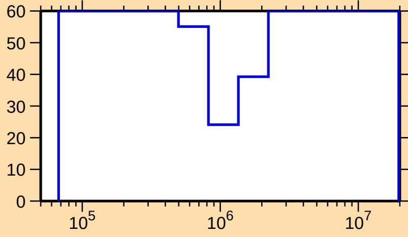
\Delta\sigma/\sigma vs. E for ^{132}\text{Cs}(n,n_1)
