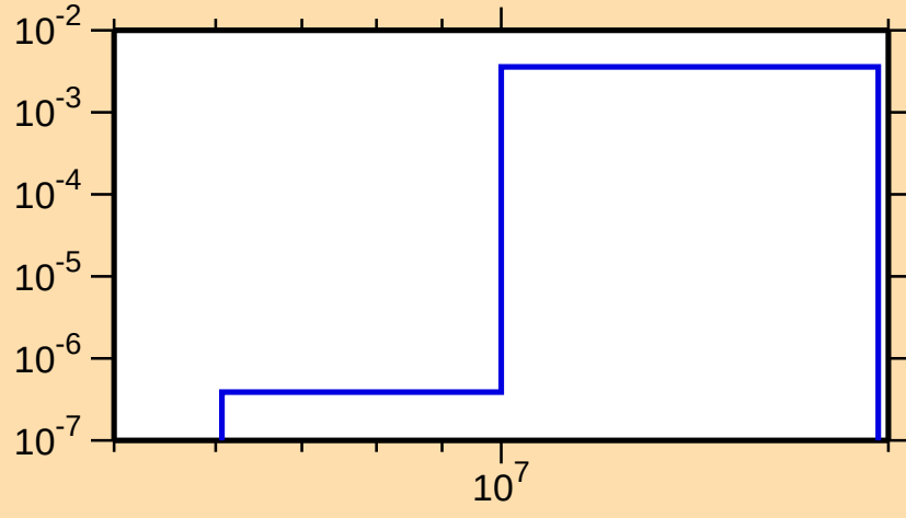
\sigma vs. E for ^{132}\text{Cs}(n,np)
