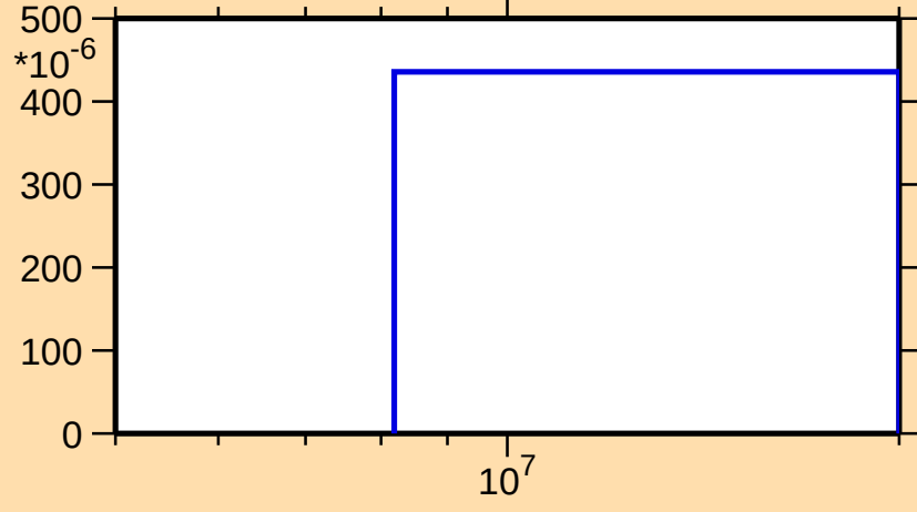
\sigma vs. E for ^{132}\text{Cs}(n,3n)
