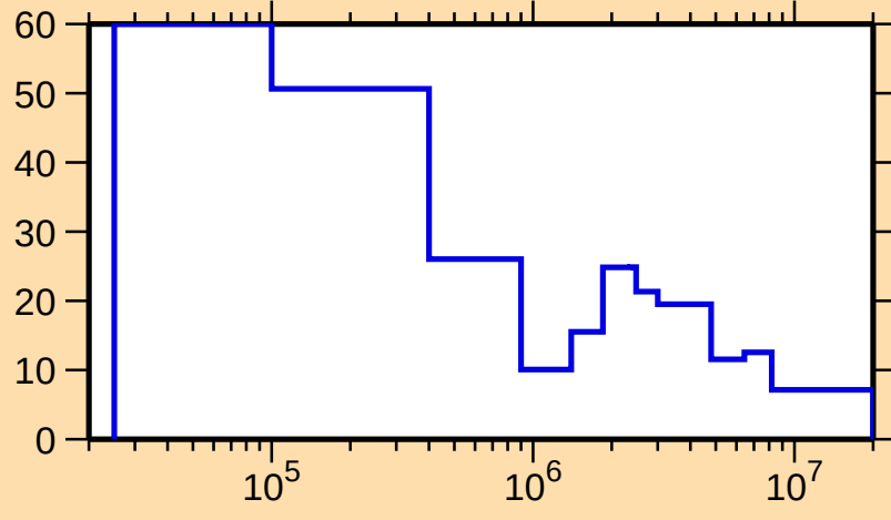
\Delta\sigma/\sigma vs. E for ^{132}\text{Cs}(n,\text{el.})
