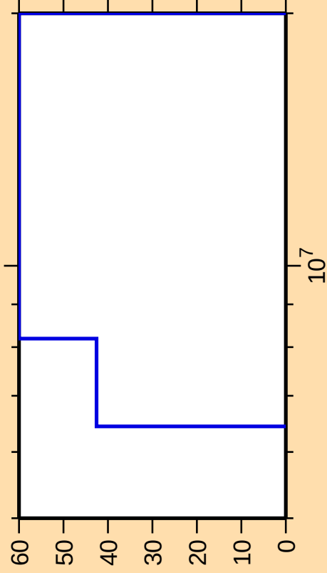
\Delta\sigma/\sigma vs. E for ^{132}\text{Cs}(n,t)
