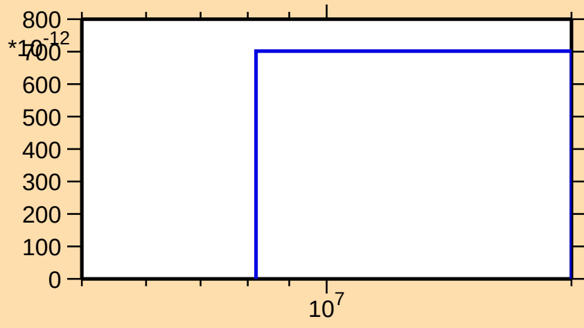
\sigma vs. E for ^{132}\text{Cs}(n,\text{He}3)
