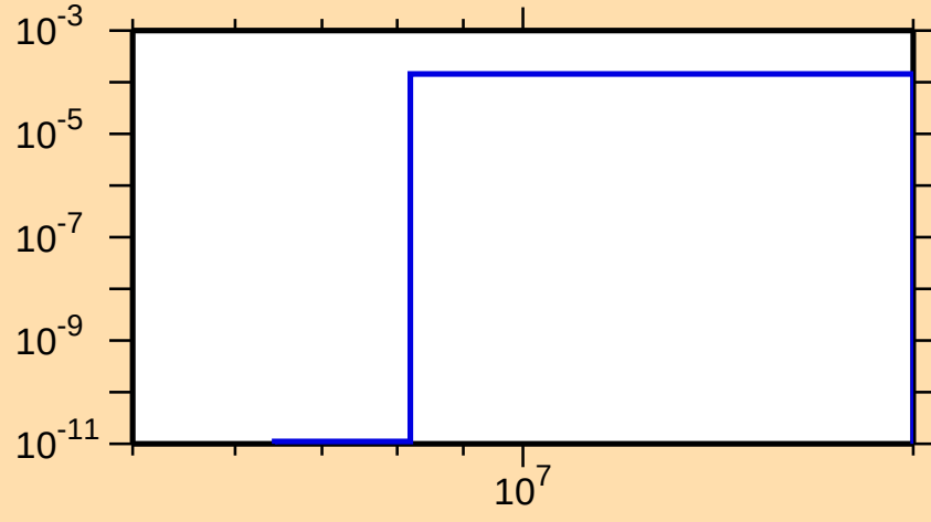
\sigma vs. E for ^{132}\text{Cs}(n,t)
