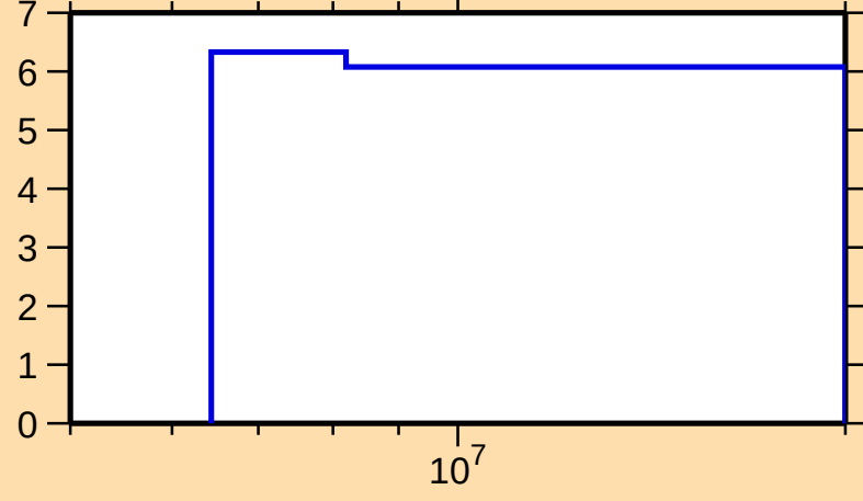
\Delta\sigma/\sigma vs. E for ^{132}\text{Cs}(n,\text{nonel.})
