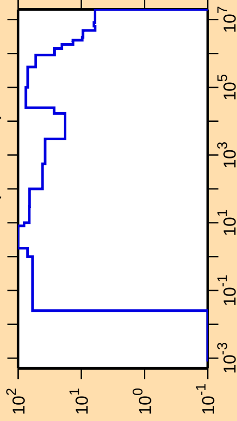
\Delta\sigma/\sigma vs. E for ^{132}\text{Cs}(n,\text{nonel.})
