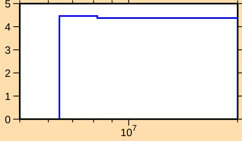
\Delta\sigma/\sigma vs. E for ^{132}\text{Cs}(n,\text{tot.})
