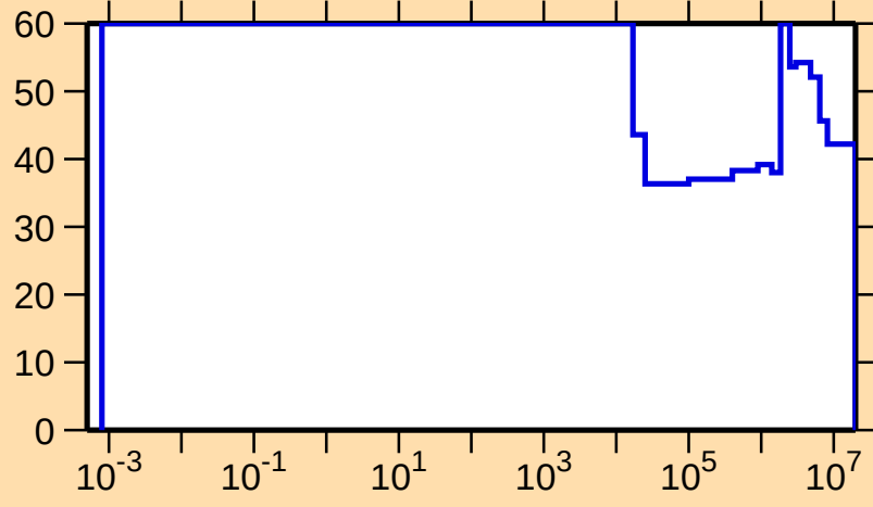
\Delta\sigma/\sigma vs. E for ^{132}\text{Cs}(n,p)
