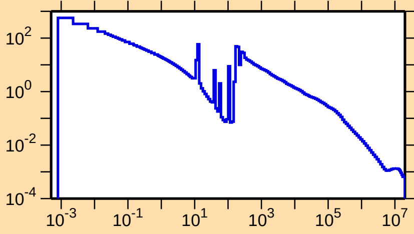
\sigma vs. E for ^{134}\text{Cs}(n,\gamma)
