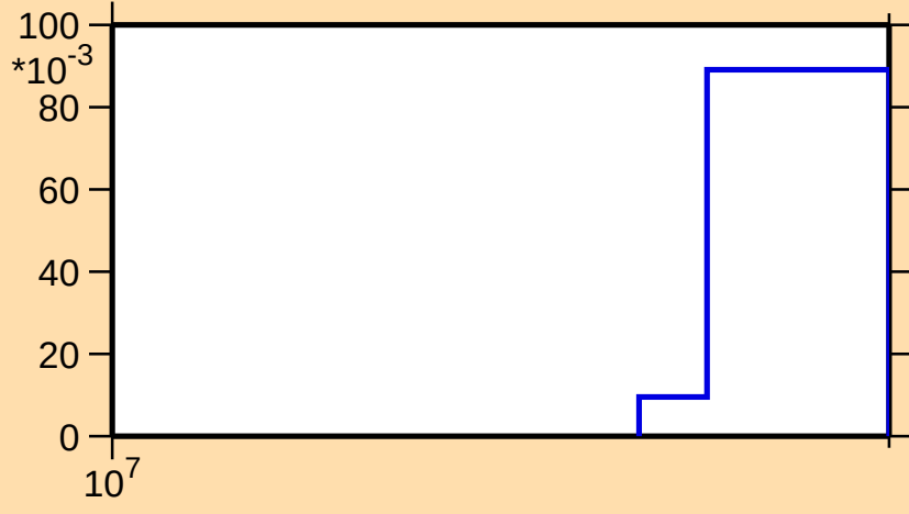
\sigma vs. E for ^{134}\text{Cs}(n,3n)
