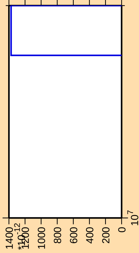
\Delta\sigma/\sigma vs. E for ^{134}\text{Cs} (mt 11)
