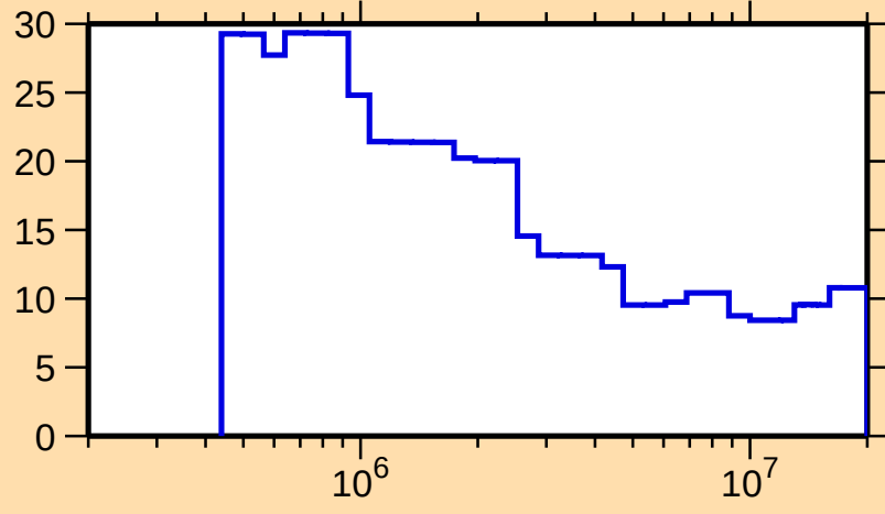
\Delta\sigma/\sigma vs. E for ^{134}\text{Cs}(\text{n},\text{nonel.})
